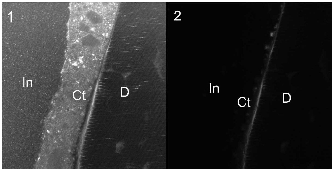
Figure 3. Representative confocal scanning micrographs of fluorescence evaluation of an unloaded, etched Panavia F 2.0 axial wall specimen. (1): Reflection (546-nm illumination). (2): Fluorescence (546/600-nm excitation/emission) images of an area of axial wall. In, inlay; Ct, resin cement; D, dentin 20/0.80× oil immersion objective.
