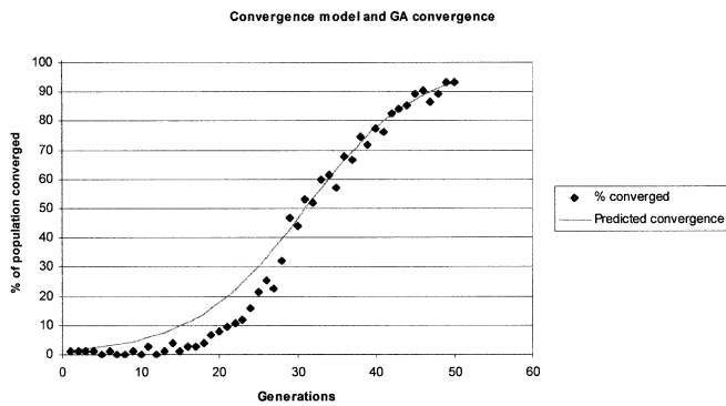
Figure 3 | Convergence model.
