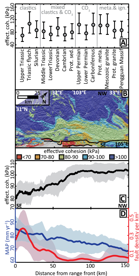
Figure 4. A: Effective cohesion (effect. coh.) with 1\sigma error bars determined from the standard derivation of mean landslide thickness for each geologic map unit (Fig. DR7; see footnote 1). The geologic map units are ordered by lithology (meta.—metamorphic; ign.—igneous; sed.—sedimentary; Prot.—Proterozoic.). B: Map view of mean effective cohesion for each geologic map unit. C, D: 300-km-wide swath profiles plotted as a function of distance from the range front. C: Mean effective cohesion (black line) and one standard error (gray area). D: Mean annual precipitation (MAP) derived from 3-arc second ( \sim 1 km) global data (Hijmans et al., 2005), and active fault density (Burchfiel et al., 1995). Lines and shaded areas show the mean and one standard error, respectively. Geologic map unit descriptions (Ministry of Geology and Mineral Resources, 1991; Burchfiel et al., 1995): Upper Triassic—siltstone, mudstone; Triassic flysch—mudstones and sandstones, low metamorphic grade; Silurian—mudstone, sandstone, marl; Middle Triassic—limestone, mudstone, local evaporites; Lower Triassic—limestone, marine clastics; Devonian—marine clastics, limestone; Cambrian—sandstone, evaporates, limestone; Proterozoic sedimentary—marine clastics, dolostone, limestone; upper and lower Permian—limestone, dolostone; Carboniferous—limestone; Proterozoic metamorphic—amphibolite-grade metasedimentary and metavolcanics; Mesozoic granite; Proterozoic granite; undifferentiated; Pengguan Massif—Proterozoic granite.
