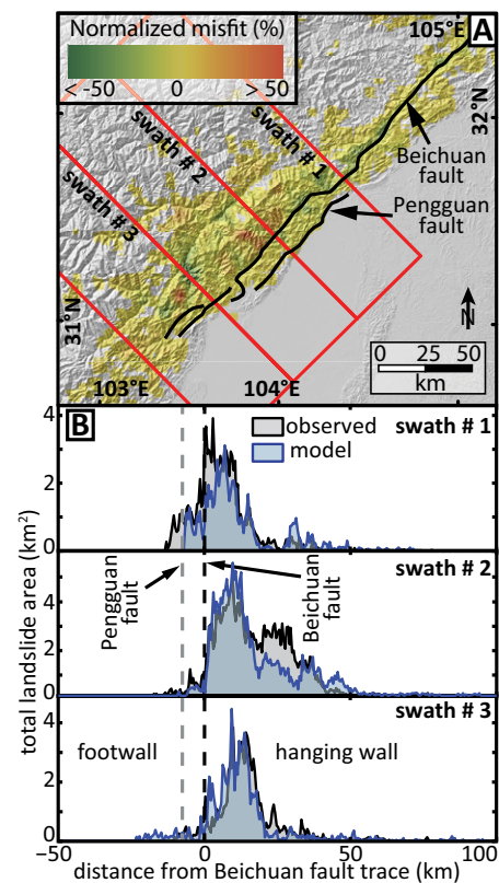
Figure 3. A: Map view of misfits between the modeled and observed landslide area densities per square kilometer, with locations of swath profiles (red boxes). B: Three \sim 50 -km-wide swath profiles of landslide area densities. Supporting data are in Figures DR5 and DR6 (see footnote 1).
