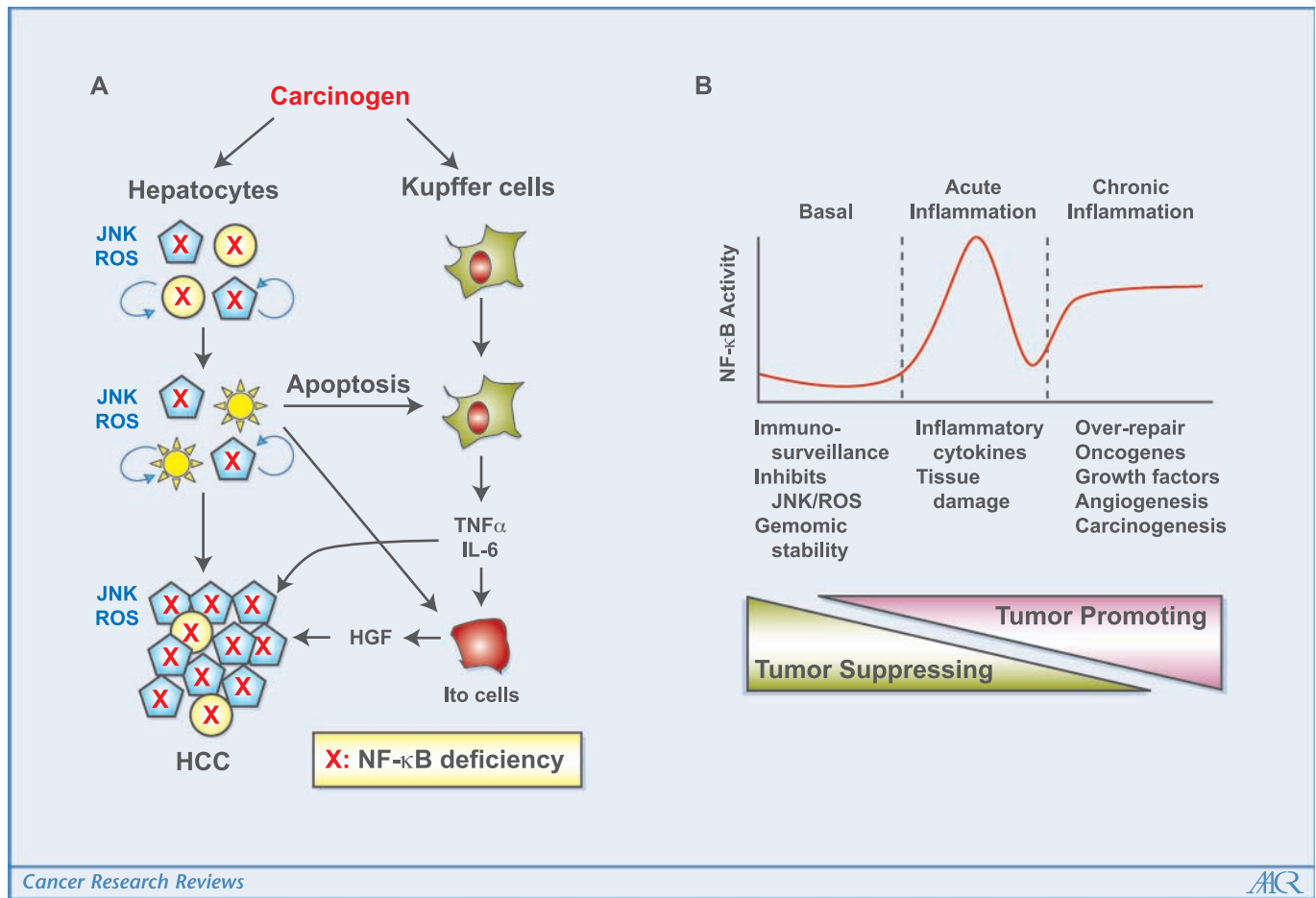
Figure 1. A, NF- \kappa B inhibition induces carcinogenesis in liver or other organs. In the liver cancer model, hepatocyte-specific deficiency (depicted by a red X) in relA , Ikk \beta , or Ikk \gamma enhances JNK activation and ROS generation in these cells. In response to a carcinogen, a subpopulation of NF- \kappa B-deficient hepatocytes undergo apoptosis because of a weakened antiapoptotic response. The apoptotic cells trigger release of hepatomitogens such as TNF \alpha and IL-6 from Kupffer cells and hepatocyte growth factor (HGF) from Ito cells in which NF- \kappa B is normal. These hepatomitogens, along with the enhanced JNK activation and ROS generation, foster uncontrolled proliferation and carcinogenic transformation of the remaining hepatocytes. These proliferative hepatocytes may be those cells that have either escaped from apoptosis despite deficiency in NF- \kappa B or differentiated into a stage that differs from that of cells prone to apoptosis (as denoted by a different shape). B, the tumor-suppressive or tumor-promoting effect of NF- \kappa B might be determined by the degree or duration of NF- \kappa B activation and other cellular contexts. The basal-level NF- \kappa B may be tumor suppressive by maintaining the functions of immunosurveillance, inhibiting JNK or ROS generation and guarding genomic stability. During acute inflammation, transient acute NF- \kappa B activation is important for inflammatory cytokine production. These cytokines may be involved in innate immune response against both invading microorganisms and tissue damage. A sustained activation of NF- \kappa B, such as in the case of chronic inflammation, is tumorigenic because of over-repair of the damaged tissues, expression of oncogenes and growth factors, and the release of a number of angiogenic factors.
