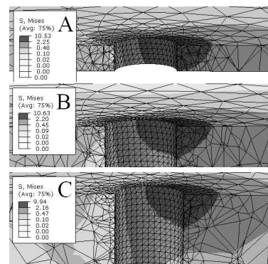
Figure 4. Von Mises stress contours in cortical bone for (A) 0.5-mm, (B) 1.0-mm, and (C) 2.0-mm cortical bone thickness.
