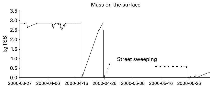
Figure 7 | Mass of TSS (kg) on the surface of the runoff plot.
