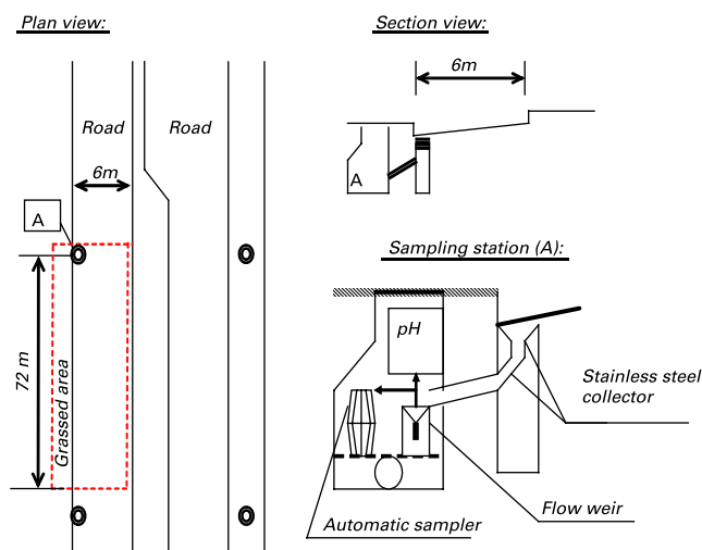
Figure 1 | Plan and section view of the runoff plot (broken lines) and the sampling station.
