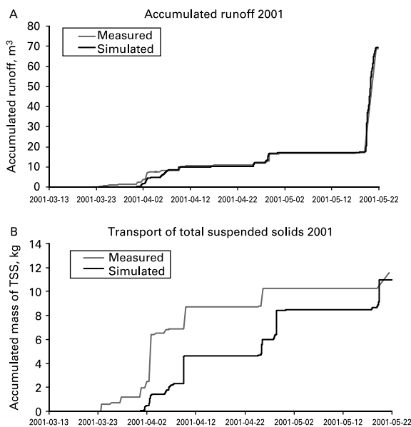
Figure 9 | Accumulated measured and modelled runoff ( \text{m}^3 ) (A) and load of TSS (kg) (B), 2001.
