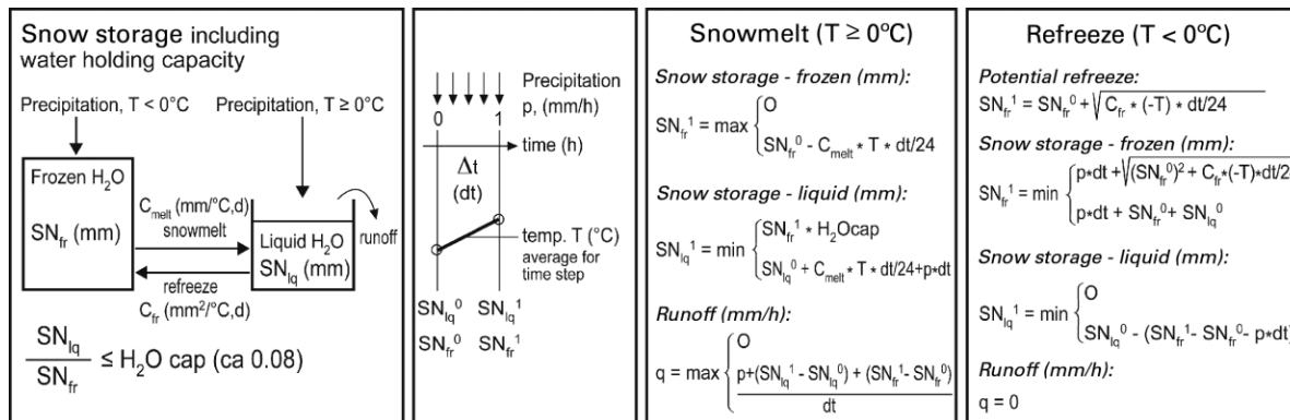
Figure 2 | Details of the model concept for runoff - modified temperature-index method (Hernebring 1996).
