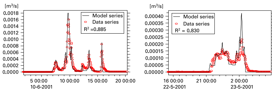
Figure 5 | Verification of contributing area during rainfall.
