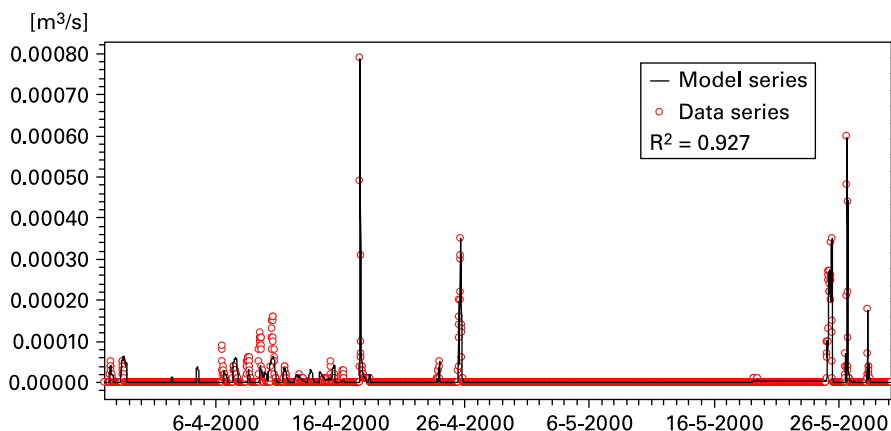
Figure 6 | Measured and modelled discharge ( \text{m}^3/\text{s} ) of road runoff during the measuring period.
