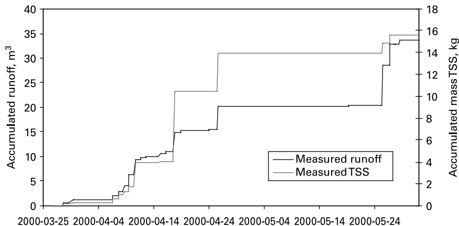
Figure 4 | Measured accumulated runoff ( \text{m}^3 ) and mass of total suspended solids (kg).
