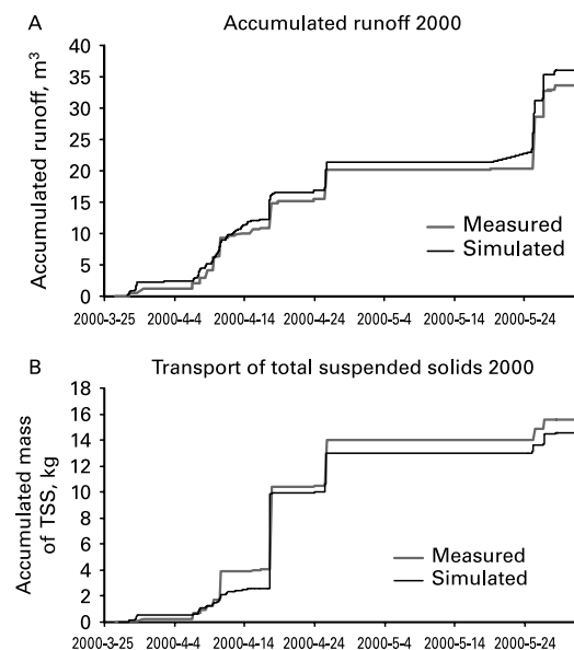
Figure 8 | Accumulated measured and modelled runoff ( \text{m}^3 ) (A) and load of TSS (kg) (B), 2000.
