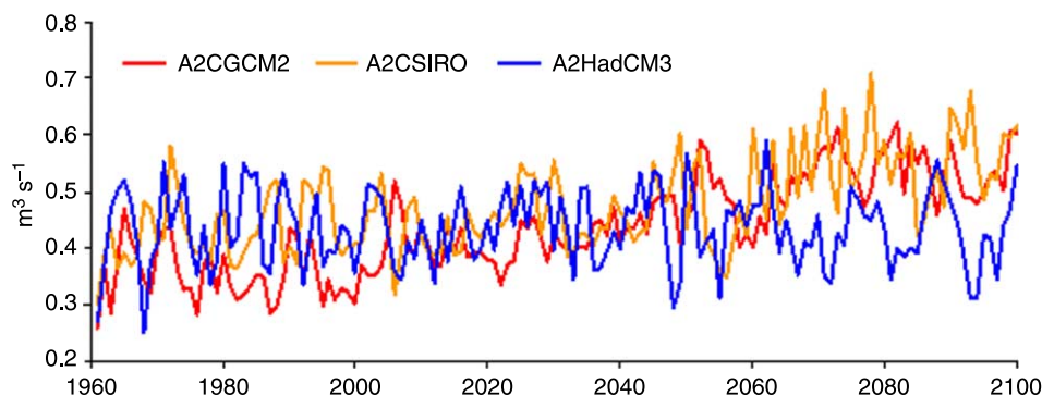
Figure 2 | Annual average river flows simulated in the River Kennet for three different GCM outputs from 1960–2100.
