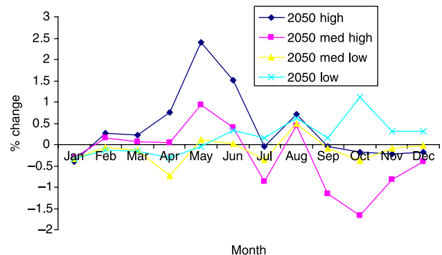
Figure 8 | Percentage changes in monthly sediment concentrations in the upper Lambourn for the 2050s.
