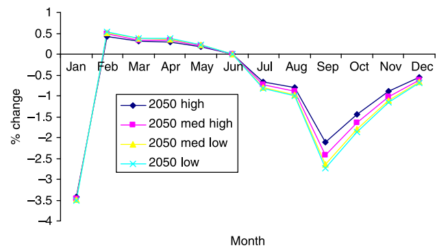
Figure 7 | Upper River Tamar monthly (%) changes in nitrate (as N) for the 2050s.
