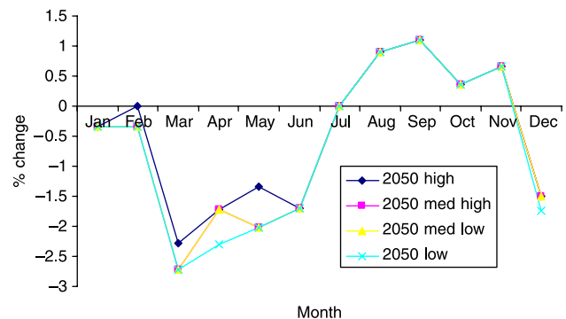
Figure 5 | River Lugg monthly (%) changes in phosphorus (SRP) for the 2050s.
