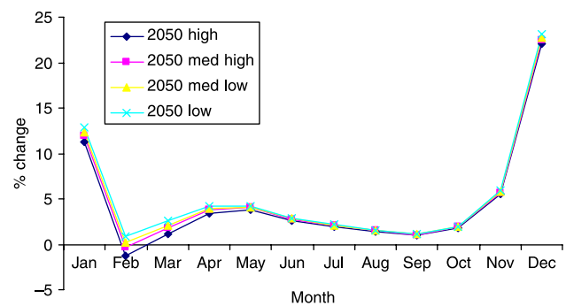
Figure 4 | River Tame monthly (%) changes in phosphorus (SRP) for the 2050s.
