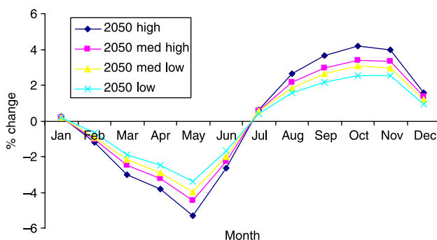
Figure 3 | Monthly (%) changes in phosphorus for the 2050s.
