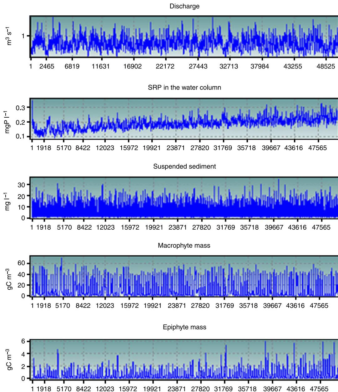
Figure 9 | Simulated flow, phosphorus (SRP), sediment, macrophyte and epiphyte biomass ( \text{gC m}^{-3} ) for the Lambourn for the A2 scenario 1961–2100 (x axis: days from 1 January 1961).
