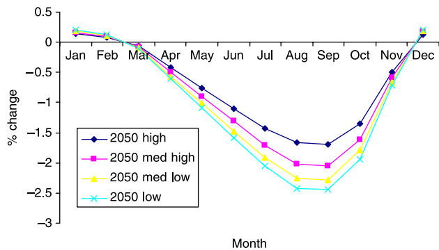
Figure 6 | River Tweed (upper reaches) monthly (%) changes in nitrate (as N) for the 2050s.
