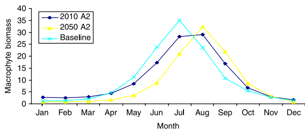
Figure 10 | Lambourn macrophyte monthly biomass ( \text{gC}\cdot\text{m}^{-2} ) for the A2 long-term scenario.
