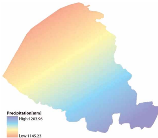
Figure 4 | Spatial distribution of summed annual precipitation in 2005.
