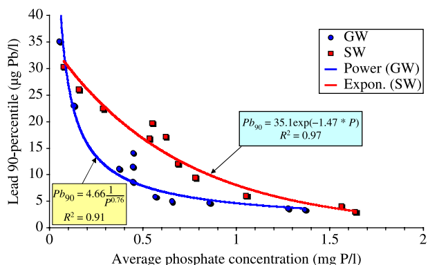
Figure 5 | Graph of annual lead 90-percentile versus average phosphate by year for surface waters (SW) and ground waters (GW).
