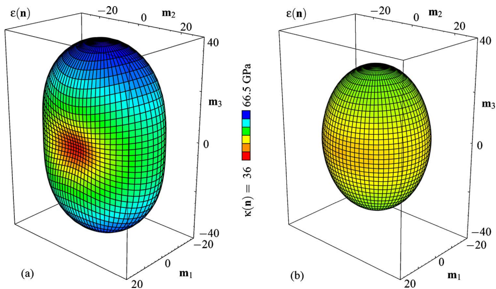
Fig. 9 Three-dimensional representation of the elongation modulus \varepsilon(\mathbf{n}) in function of a direction vector \mathbf{n} with the bulk modulus \kappa(\mathbf{n}) superimposed: the shape of the surfaces represents \varepsilon , while the color represents \kappa . (a) Mean osteon in cortical bone tissue measured by means of nanoindentation. (b) Cortical bone at the macroscopic level. Units are in [GPa].
