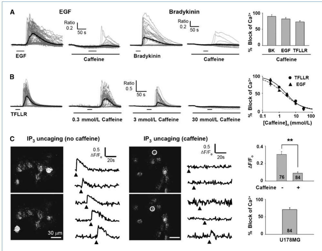
Figure 3. Caffeine reduces GPCR- and RTK-induced \text{Ca}^{2+} increase by inhibiting IP 3 R. A, EGF- or bradykinin-induced \text{Ca}^{2+} responses in the presence or absence of caffeine in U178MG cells. Caffeine (10 mmol/L) was treated 100 s before stimulation with indicated agonist. Percent block of various agonists induced \text{Ca}^{2+} release by 10 mmol/L caffeine in U178MG cells. The peak of average \text{Ca}^{2+} response trace in the presence of caffeine was divided by the average of \text{Ca}^{2+} response in the absence of caffeine ( n = 3 ). B, TFLLR-induced \text{Ca}^{2+} responses in the presence of 0.3, 3, and 30 mmol/L of caffeine. Concentration-effect curve of \text{Ca}^{2+} increase evoked by TFLLR ( \text{IC}_{50} , 2.45 mmol/L) or EGF ( \text{IC}_{50} , 1.87 mmol/L). C, left, intensity images of U178MG cells loaded with caged IP 3 and Oregon Green 488 BAPTA-2. White circles, region of interest exposed to a 405-nm laser for uncaging of IP 3 . Right traces, representative fluorescence changes on laser stimulation ( \blacktriangle ) over time in the absence of caffeine or in the presence of 10 mmol/L caffeine. The average fluorescence intensity changes in the presence or absence of caffeine at the peak of \text{Ca}^{2+} transients. **, P < 0.001 , Student's t test. Summary of IP 3 uncaging experiment. Caffeine blocks 71% of \text{Ca}^{2+} release in U178MG cells.
