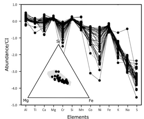
Figure 2. Bulk compositions of urban cosmic spherules showing abundances of elements compared to CI chondrite, and major element compositions (in wt%) (inset) compared to Antarctic micrometeorites (gray; Genge et al., 1997).
