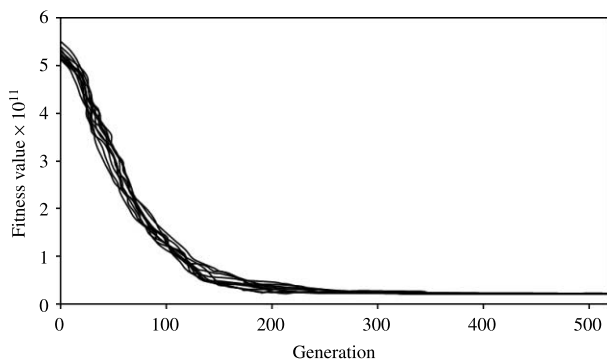
Figure 10 | Rate of convergence of the fitness function for 10 runs of the PSO.
