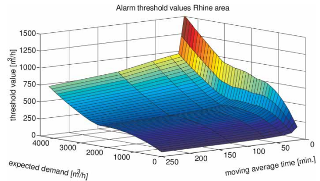
Figure 9 | Alarm threshold values for the expected water demand in the Rhine area.
