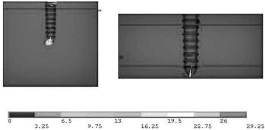
Figure 7. Von Mises stress (MPa) in nonosseointegrated configurations subjected to a load of 240 g.
