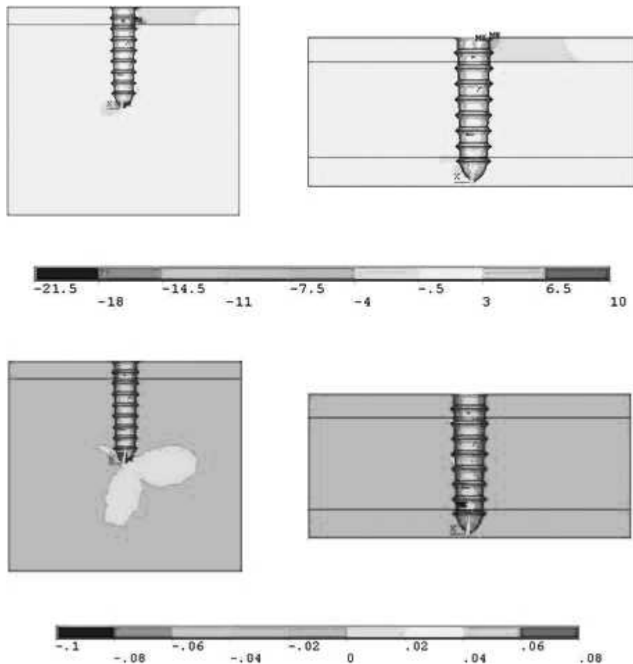
Figure 8. Stress \sigma_x in MPa (above) and strain \epsilon_x (below) for the nonosseointegrated configurations loaded with 480 g.
