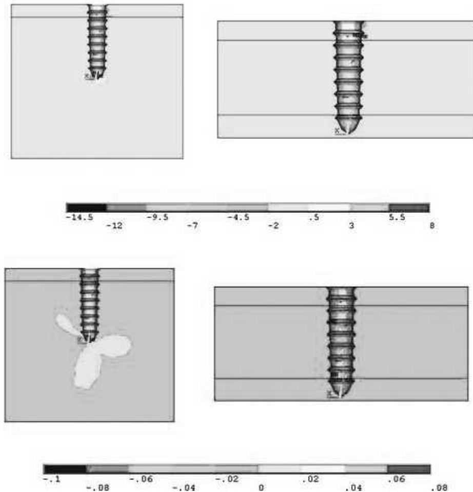
Figure 6. Stress \sigma_x in MPa (above) and strain \varepsilon_x (below) for the nonosseointegrated configurations loaded with 240 gf.
