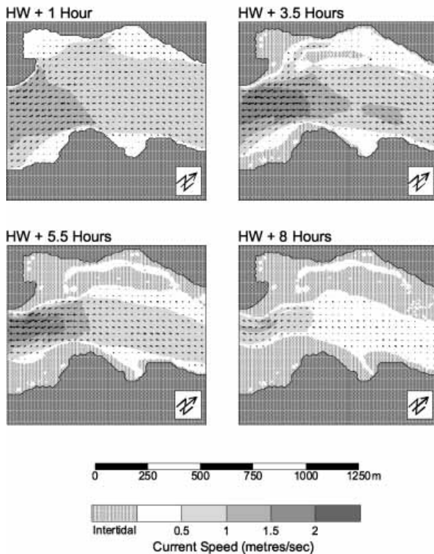
Figure 9 | Surface current velocities: River Taw.
