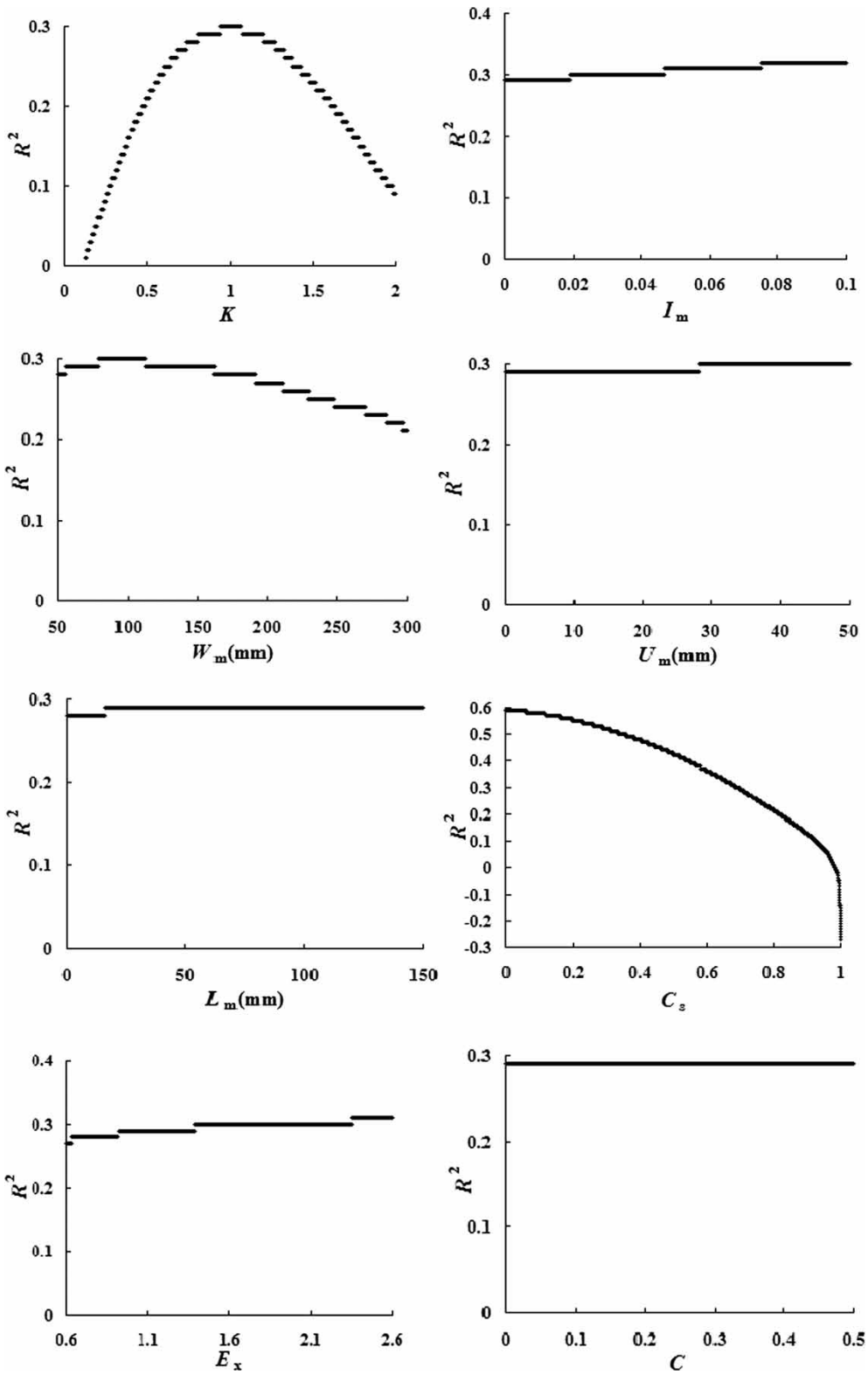
Figure 3 | Sensitivity of Xinanjiang model parameters in water balance parameter calibration (continued).
