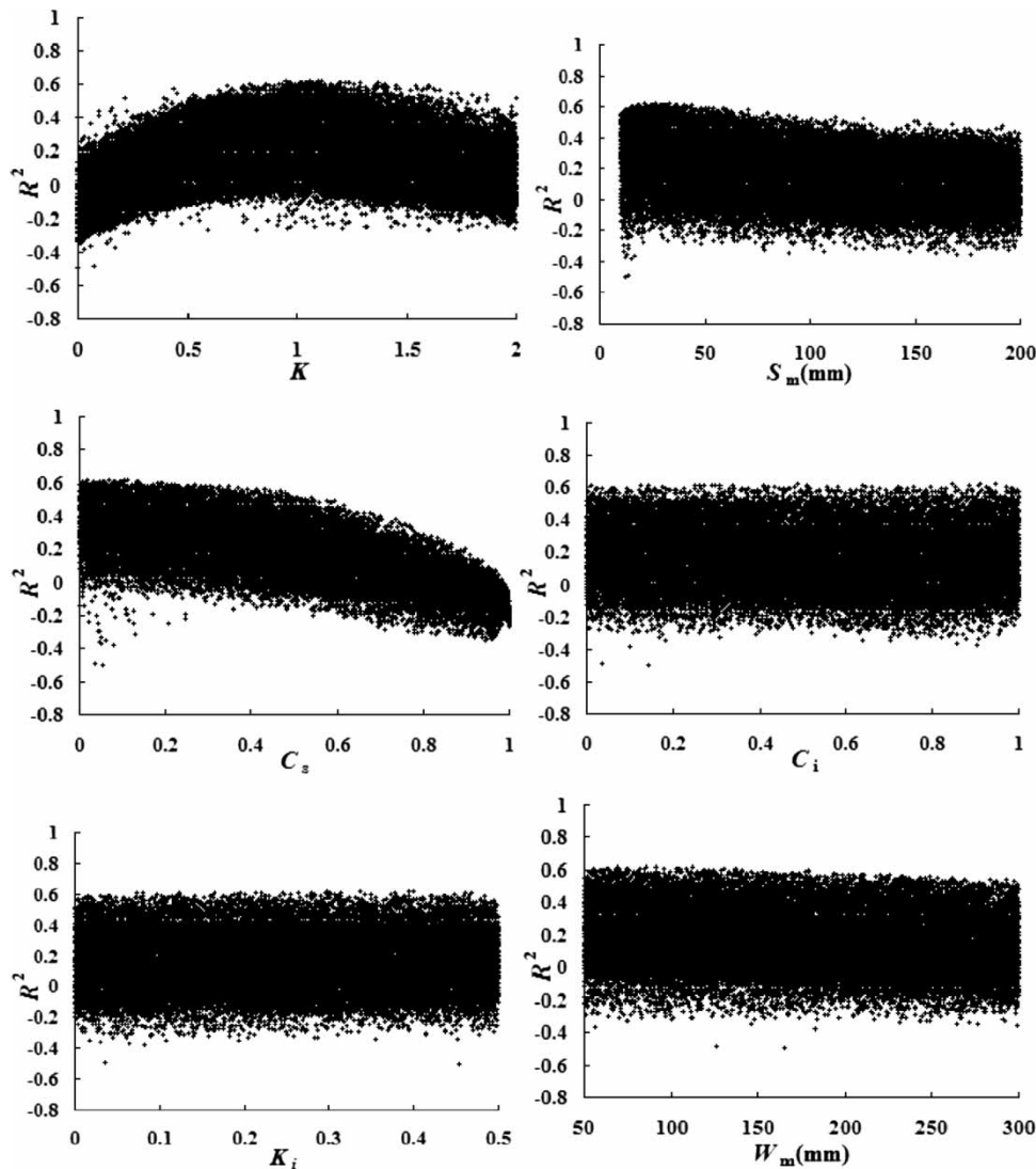
Figure 4 | Scatter plots of the likelihood of some sensitive Xinanjiang model parameters in water balance parameter calibration.
