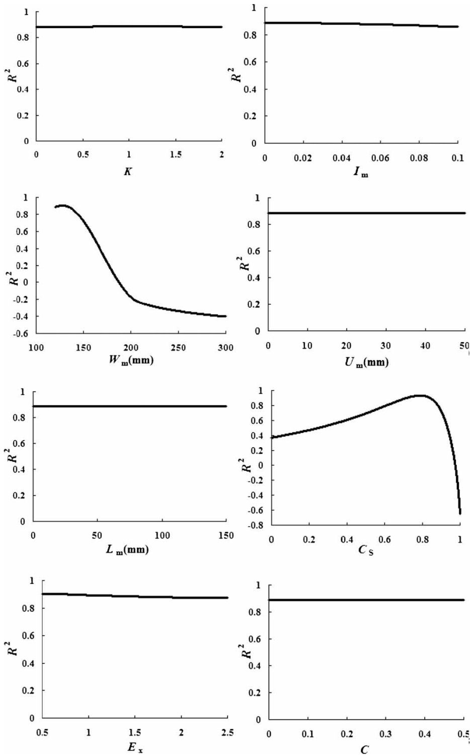
Figure 5 | Sensitivity of Xinanjiang model parameters in runoff routing parameter calibration (continued).
