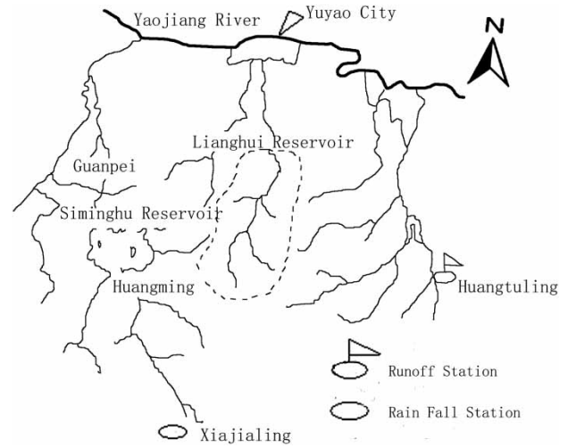
Figure 2 | Distribution of hydrological stations around LiangHui reservoir.
