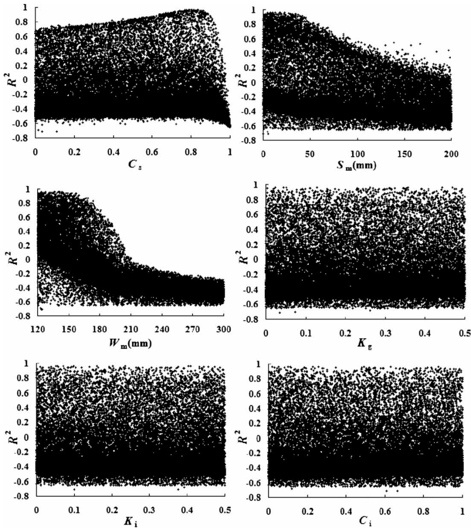
Figure 6 | Scatter plots of the likelihood of some sensitive parameters in runoff routing parameter calibration.
