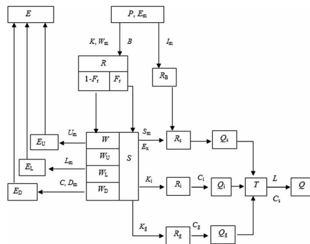
Figure 1 | Structure of the Xinanjiang model (Zhao 1984).
