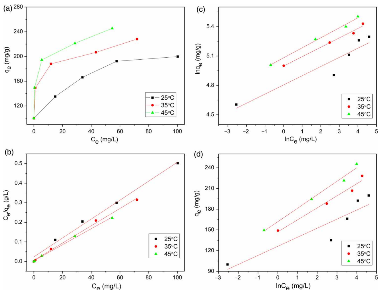
Figure 4 | (a) The plot of adsorption capacity against equilibrium concentration of Cr(VI); (b) Langmuir adsorption isotherm, (c) Freundlich adsorption isotherm, and (d) Temkin isotherm for Cr(VI) ion adsorption on PANI/sepiolite nanofibers.
