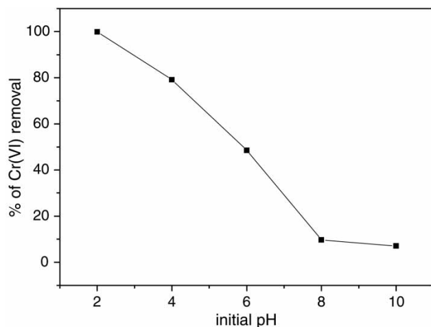
Figure 2 | Effect of pH on the adsorption of Cr(VI) by PANI/sepiolite nanofibers (PANI/sepiolite dose 1 g/L; initial Cr(VI) 200 ppm; time 3 h).
