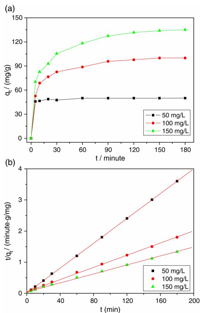
Figure 3 | (a) Adsorption kinetic curves and (b) pseudo-second-order kinetic plots for the adsorption of Cr(VI) at different initial concentrations.
