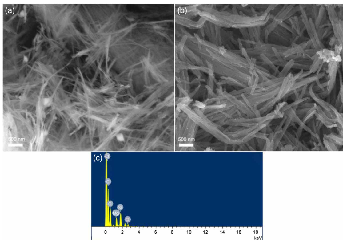
Figure 1 | (a) SEM image of sepiolite; (b) SEM and (c) EDX images of PANI/sepiolite.
