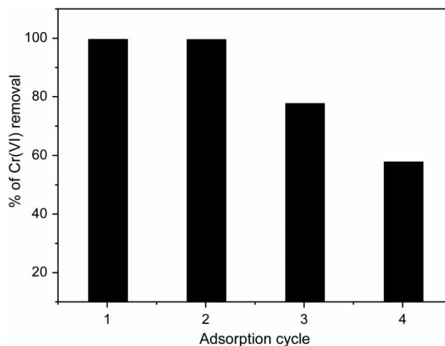
Figure 5 | Regeneration of PANI/sepiolite for four cycles.
