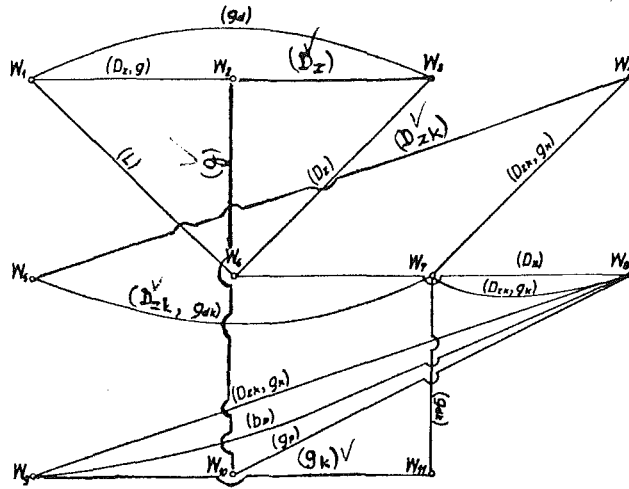
Fig. 2 The constraint graph for the boiler drum
