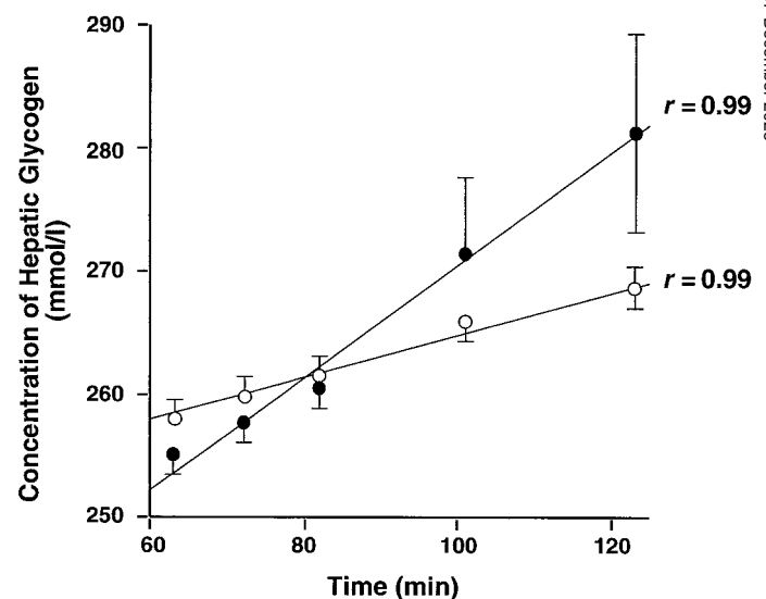
FIG. 2. Rates of net hepatic glycogen synthesis in humans under euglycemic (5 mmol/l) hyperinsulinemic (400 pmol/l) conditions. □, Control studies; ■, fructose studies.
