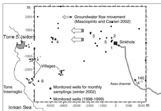
Figure 3 | Asso Channel, sinkhole and location of the affected community in the villages and Torre S. Isidoro town. The monitoring wells #1, #2, #3, #4 and #5 were selected for monthly sampling during winter 2002. Well #2 was used for the hypochlorination test. Well #6 was used for village tap water tests.
