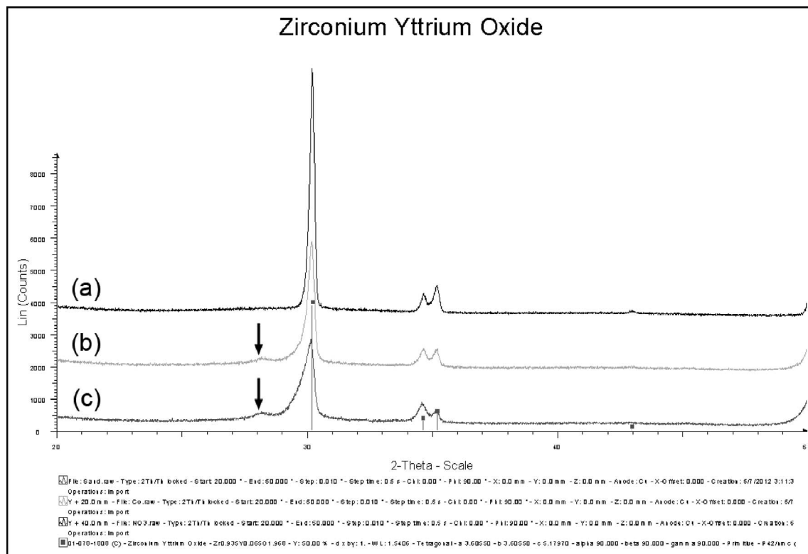
Figure 5. XRD results after air-abrasion and CoJet treatment on zirconia surfaces: (a) control; (b) surface coated with 30 \mu\text{m} silica-modified \text{Al}_2\text{O}_3 particles; and (c) surface air-abrasion with 50 \mu\text{m} \text{Al}_2\text{O}_3 . The arrows indicate monoclinic phase transformation.
