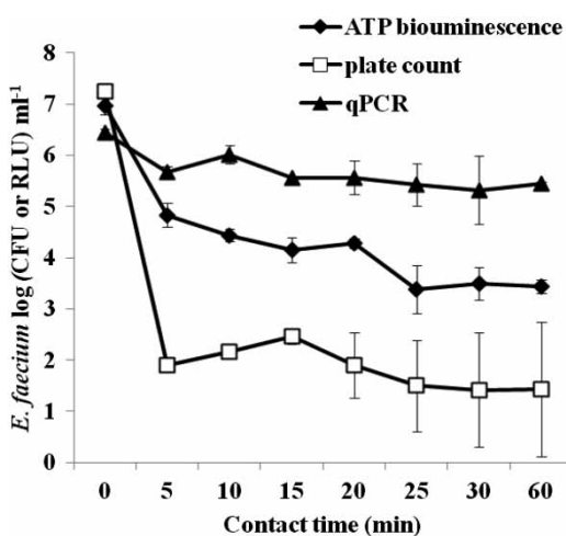
Figure 1 | Concentration of the surviving E. faecium measured with three methods when treated with PAA (5 ppm) during 1-h contact time: ATP bioluminescence (log RLU mL -1 ), plate count (log [CFU] mL -1 ), qPCR (log [CFU] mL -1 ).
