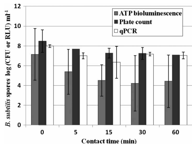
Figure 2 | Concentration of the surviving B. subtilis spores measured with three methods when treated with PAA (500 ppm) during 1-h contact time: ATP bioluminescence (log RLU mL -1 ), plate count (log [CFU] mL -1 ), qPCR (log [CFU] mL -1 ).
