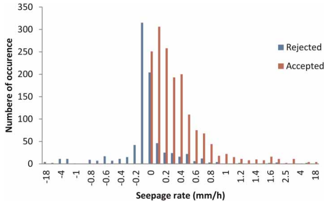
Figure 9 | Frequency of seepage rate for all gauges in 2010–11 using linear regression.
