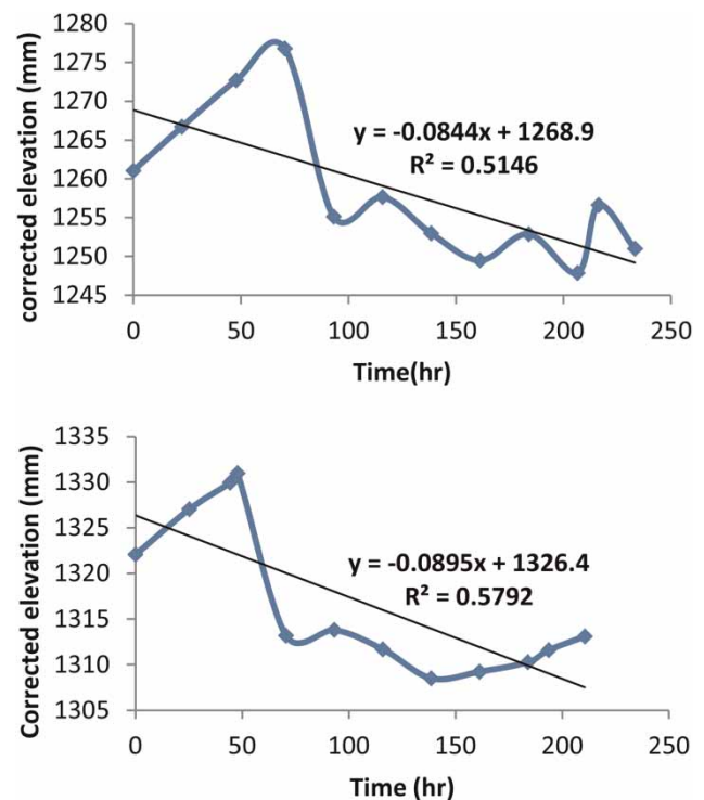
Figure 4 | Example of a pool classified in group 4.
