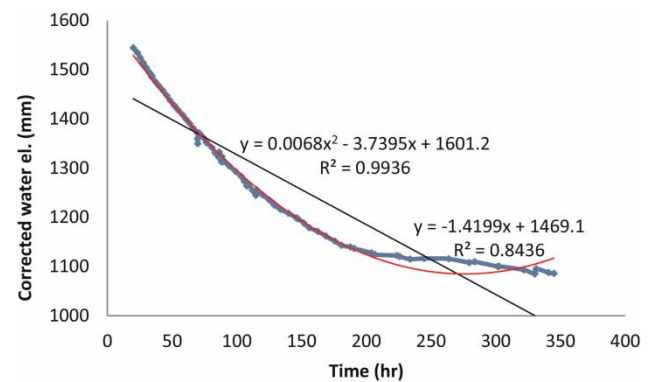
Figure 10 | Application of polynomial and linear regression trend line to ideal seepage curve.
