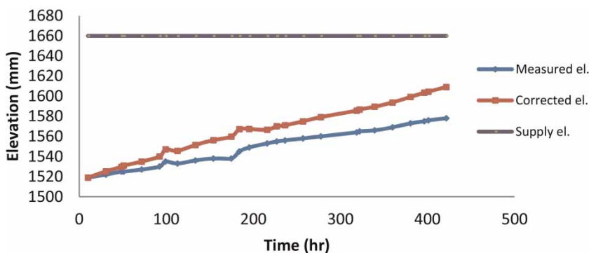
Figure 5 | Pondage showing a continuous increase in measured water elevations.
