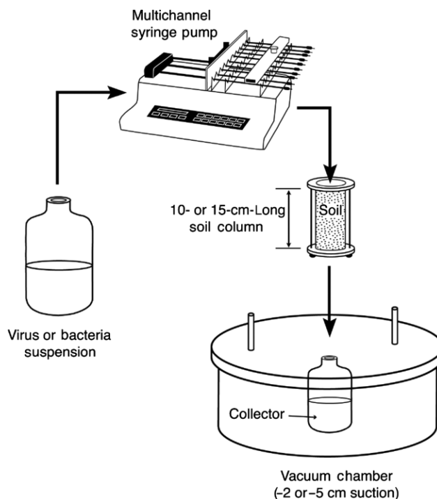
Figure 1 | Experimental setup for a leaching column. Leaching solutions are collected in sterile containers.
