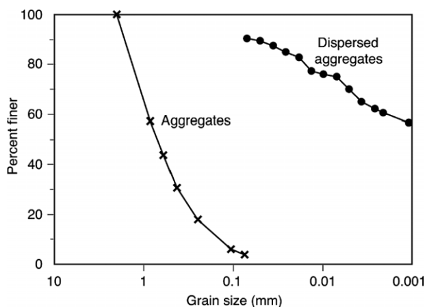
Figure 2 | Grain-size distribution of intact and dispersed aggregates in water. The plot to the left is determined by conducting a sieve of aggregated soil in a nest of sieves and that to the right is for dispersed aggregates in water.
