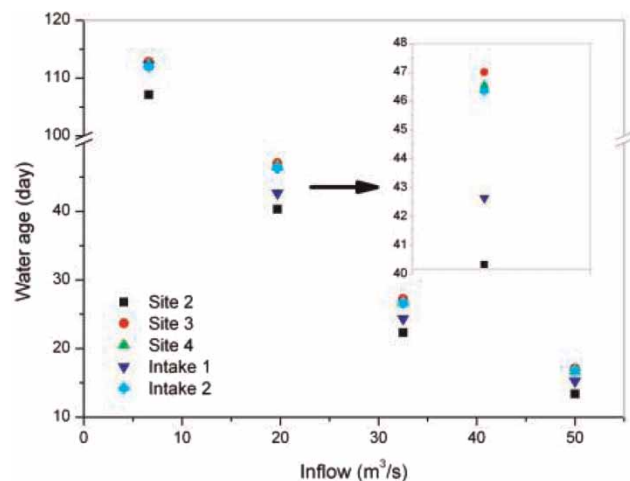
Figure 10 | Influence of inflow on water age for different scenarios (cases 2–5).
