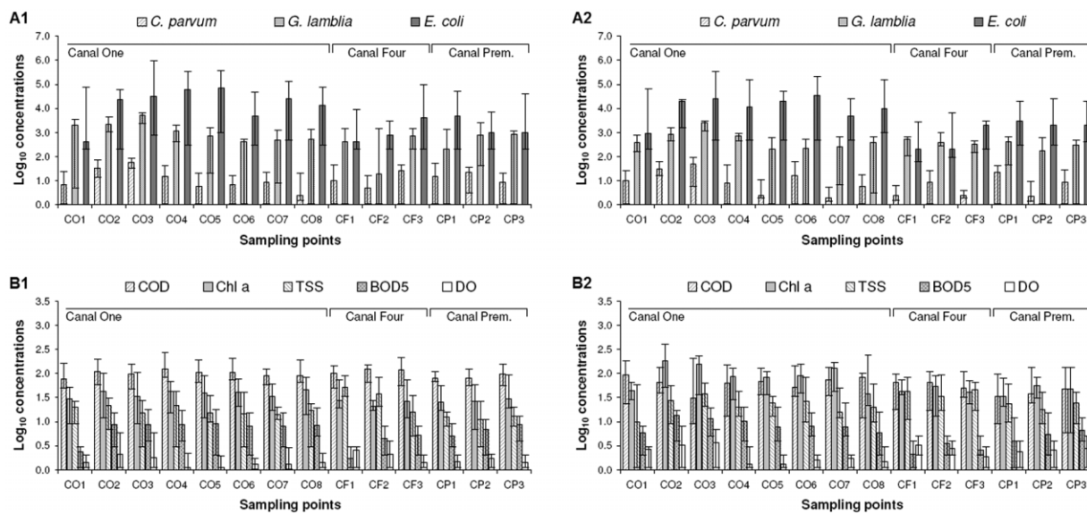
Figure 3 | Median log 10 concentrations of the pathogens (A1, A2 → rainy, dry season) and physico-chemical parameters (B1, B2 → rainy, dry season) in water columns. Line bars (+/–) represent 95% confidence interval. Parameters: chemical oxygen demand (COD, mg/l), five-day biological oxygen demand (BOD 5 , mg/l), total suspended solids (TSS, mg/l), chlorophyll a (Chl a , μg/l), dissolved oxygen (DO, mg/l), C. parvum (oocysts/l), G. lamblia (cysts/l), E. coli (MPN/100 ml); see Table 1 for the canal name abbreviations.
