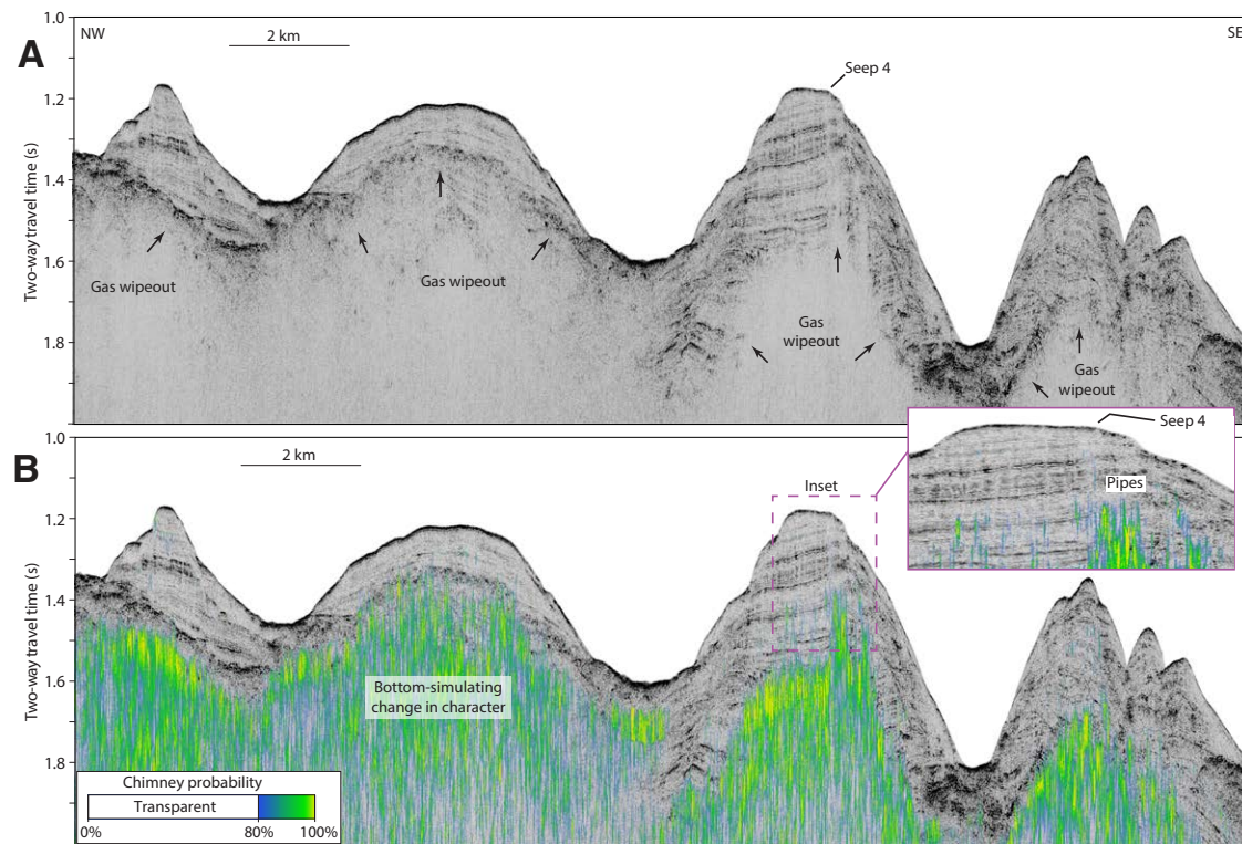
Figure 3. (A) Multichannel seismic reflection profile (see Fig. 2A for location) crossing a series of intercanyon ridges and seep 4 (vertical exaggeration 7×). Black arrows delineate the top of the acoustic wipeout zone. (B) Chimney meta-attribute overlay showing only the highest-probability (>80%) chimney detections. Note the bottom-simulating change in acoustic character and disrupted reflectors, or pipes, that extend subsection from the gas-wipeout zone to the seep site.
