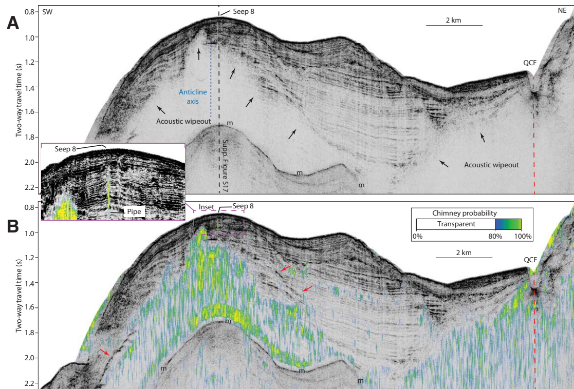
Figure 5. (A) Multichannel seismic reflection profile (see Fig. 2B for location) crossing seep 8 and the axis of a buried anticline (vertical exaggeration 6x) (see a crossing line in Fig. S17 [text footnote 1]). (B) Chimney meta-attribute overlay showing only the highest-probability (>80%) chimney detections. Note the acoustic-wipeout zone (black arrows) that extends upsection toward the seep site; the enlarged inset shows a series of vertical pipes illuminated by high chimney probabilities. Red arrows denote a series of reverse-polarity reflections that appear to be bottom simulating. The seafloor multiple (m) is a data artifact. QCF—Queen Charlotte fault.
