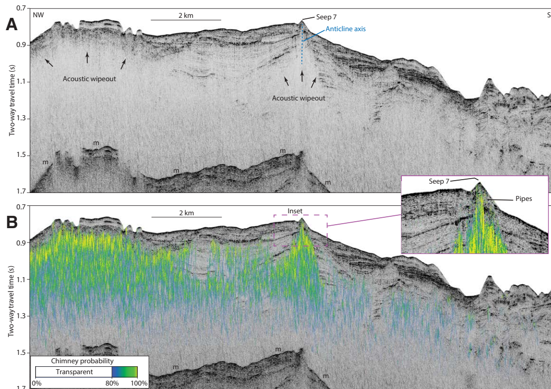
Figure 4. (A) Multichannel seismic reflection profile (see Fig. 2B for location) crossing seep 7 and the axis of a buried anticline (vertical exaggeration 7x). (B) Chimney meta-attribute overlay showing only the highest-probability (>80%) chimney detections. Note the acoustic-wipeout zone (black arrows) that extends upsection toward the seep site; the enlarged inset shows a series of vertical pipes illuminated by high chimney probabilities. The seafloor multiple (m) is a data artifact.
