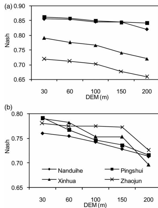
Figure 9 | Nash values under different DEM resolution during (a) calibration period and (b) validation period.
