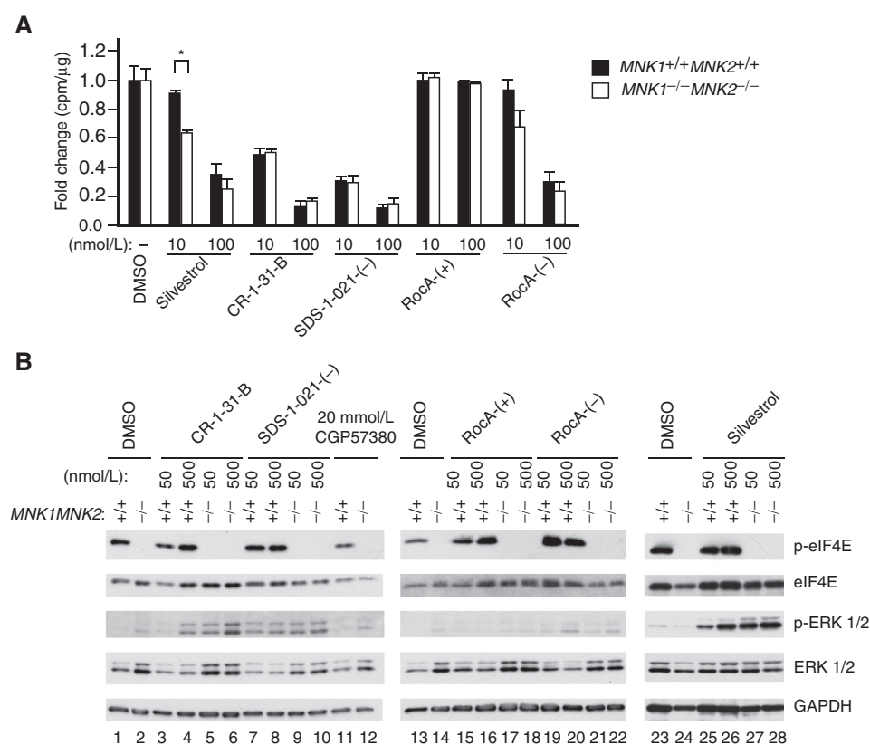
Figure 3. A, rocaglates inhibit translation in MNK1 +/+ MNK2 +/+ and MNK1 -/- MNK2 -/- MEFs. Protein synthesis rates were determined as described in Materials and Methods. The relative rates of 35 S-Met incorporation are normalized to DMSO. n = 4; error bars, error of the mean. *, P < 0.001 (Student t test). B, effects of rocaglates on eIF4E phosphorylation in MNK1 +/+ MNK2 +/+ and MNK1 -/- MNK2 -/- cells. Cells were incubated in the presence of the indicated compounds for 2 hours, lysed, resolved on a 10% polyacrylamide gel, and transferred to PVDF membranes for Western blotting. Blots were probed with antibodies directed to the proteins indicated to the right of the panel. GAPDH levels were used as an internal standard to account for variations in extract levels between lanes. Note that lane 24 is slightly underloaded based on the GAPDH internal standard.
