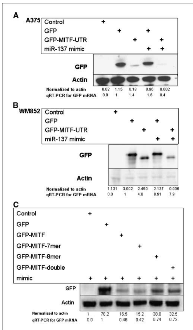
Figure 3. MITF is regulated through its 3'UTR. A , A375 cells were transfected with GFP or GFP-MITF-3'UTR plasmids with or without a mimic of miR-137. Shown is GFP protein expression measured by Western blot analysis and compared with a loading control of \beta -actin. GFP protein expression was down-regulated in cells containing the MITF-3'UTR and further down-regulated in cells with the MITF-3'UTR and the miR-137 mimic. Quantitative RT-PCR (qRT-PCR) of GFP compared with \beta -actin confirmed transfection. B , WM852 cells, which express high levels of MITF, were transfected as described above and examined for GFP protein expression by Western blot analysis and compared with a loading control of \beta -actin. The expression of the GFP-MITF-3'UTR decreased dramatically with the addition of mimic to miR-137. GFP proteins generated from the GFP-MITF-3'UTR plasmid are slightly smaller than the empty vector control because of an altered stop codon. C , A375 cells were transfected with GFP, GFP-MITF-3'UTR, GFP-MITF-7mer, GFP-MITF-8mer, GFP-MITF-double mutant plasmids, and miR-137 mimic. GFP protein expression was down-regulated in those cells with a functional MITF-3'UTR. Mutation of the 8-mer binding site in the GFP-MITF-3'UTR (GFP-MITF-8mer or GFP-MITF-double) blocked the suppression of GFP-MITF-3'UTR construct. Quantitative RT-PCR of GFP compared with \beta -actin confirmed transfection; however, as previously shown, GFP-MITF-UTR message is also reduced, suggesting that the mimic causes degradation of the message as well as the protein.
