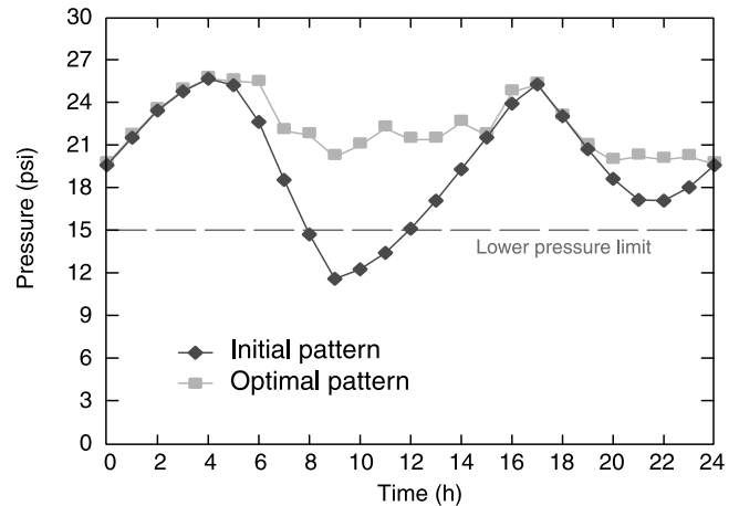
Figure 6 | Water pressure at junction #3,399 using two different patterns, May 1962 (from Maslia et al. 2001).
