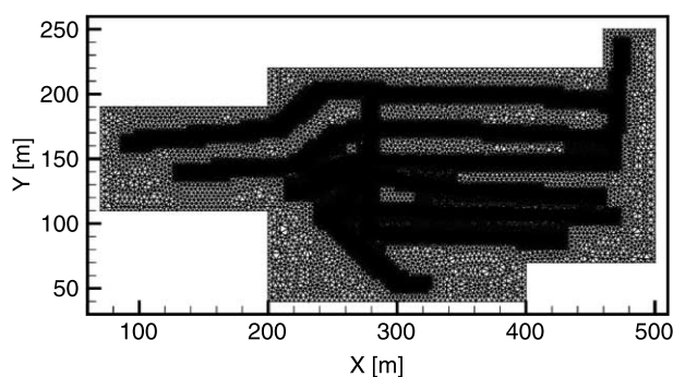
Figure 9 | Generated mesh including the surrounding coal seams.
