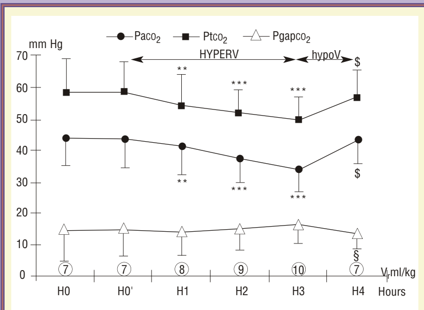
Figure 5 Changes in P_{aCO_2} , gastric intramucosal carbon dioxide tension ( P_{tCO_2} ), and gastric-arterial carbon dioxide tension difference ( P_{gapCO_2} ) induced by hourly modifications of alveolar ventilation level. Progressive increase in tidal volume (HYPERV = hyperventilation). Note the significant decrease in P_{aCO_2} and the concurrent decrease in P_{tCO_2} , such that the gap ( P_{gapCO_2} ) remains essentially unchanged. During a decrease in tidal volume (hypoV = hypoventilation) both the P_{aCO_2} and the P_{tCO_2} increase in a parallel fashion.
