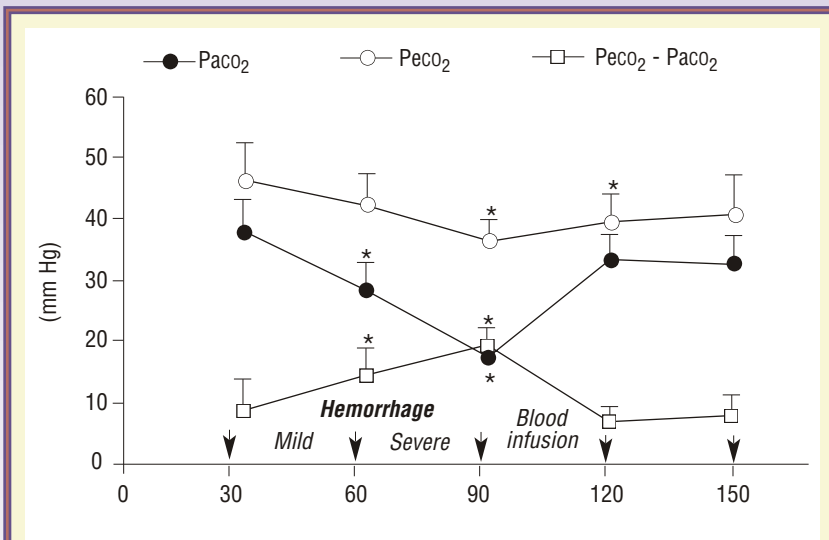
Figure 6 Changes in P_{aCO_2} , partial esophageal carbon dioxide tension ( P_{eco_2} ), and esophageal-arterial gap in 7 anesthetized, spontaneously breathing rats subjected to mild and severe hemorrhagic hypotension followed by blood reinfusion ( P < .05 with the baseline as control).
