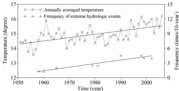
Figure 7 | Annual average temperature and frequency of flood and drought events in Huaihe River Basin from 1951 to 2006.
