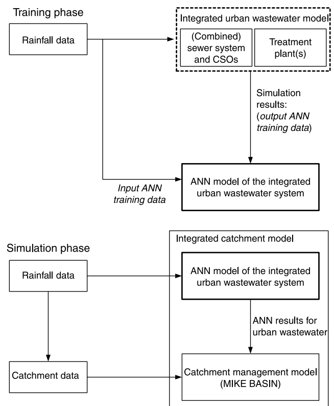
Figure 1 | Scheme of the proposed approach for modelling urban areas in a catchment scale model.
