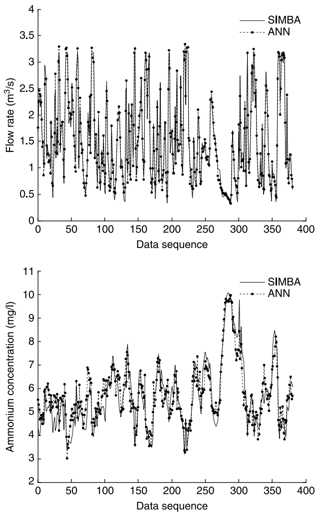
Figure 3 | ANN predictions of treatment plant effluent.
