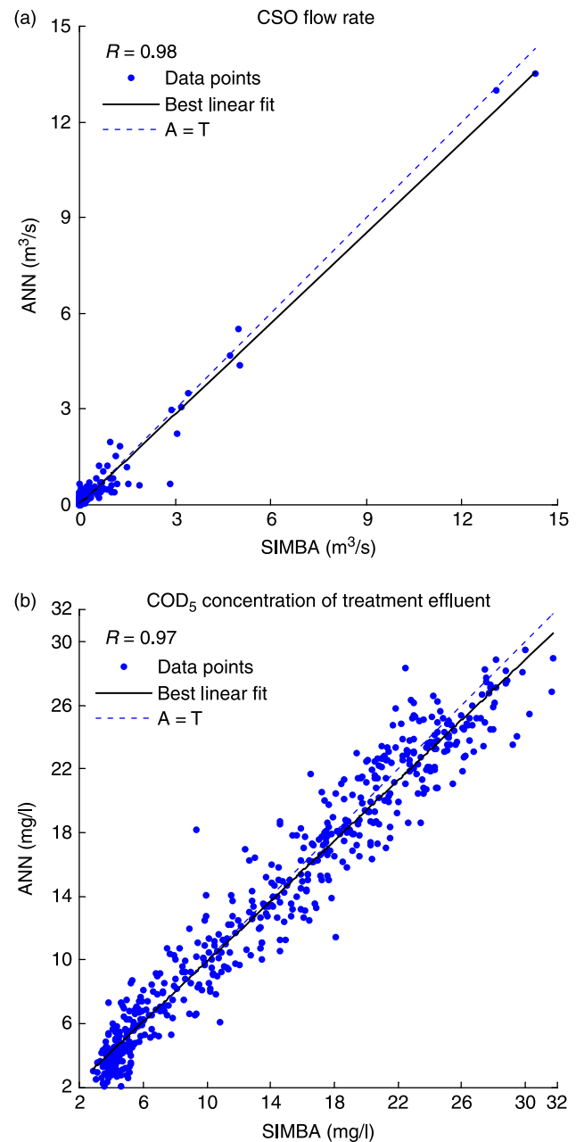
Figure 4 | Correlation between ANN predictions and SIMBA model outputs. Dotted line represents the perfect fit, i.e. ANN predictions (A) equal to targets (T).
