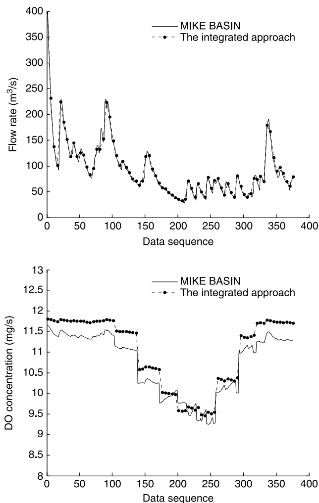
Figure 6 | Comparison results of flow and DO concentrations at downstream node N5.
