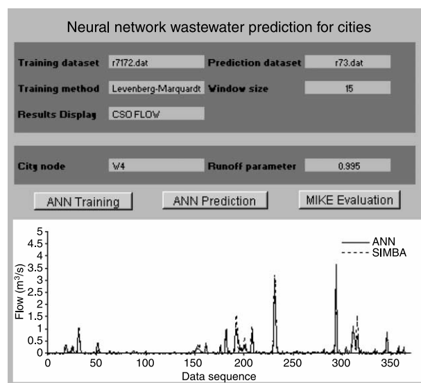
Figure 5 | Graphical user interface of the ANN predictions for city nodes.
