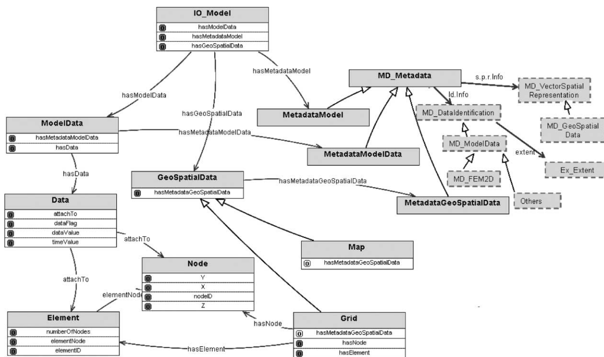
Figure 1 | Data and metadata ontology for hydrodynamic codes.
