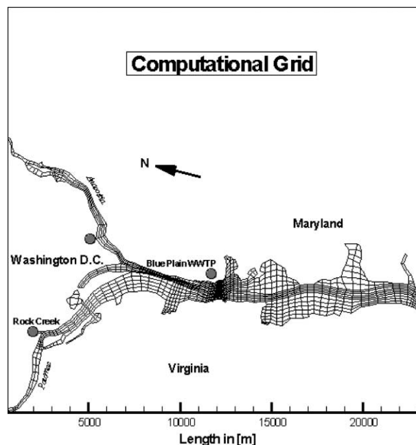
Figure 3 | Numerical grid of the Upper Potomac River.
