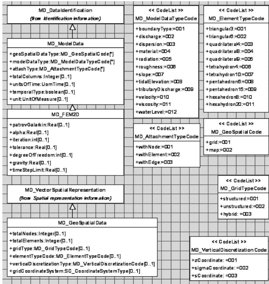
Figure 2 | List of ISO 19115 metadata extensions and code lists for hydrodynamic codes.
