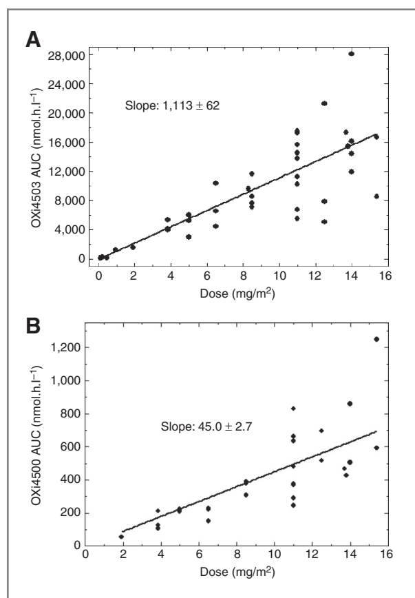
Figure 2. OXi4503 pharmacokinetics. Relationships between dose (in \text{mg/m}^2 ) and area under the curve (AUC; in \text{nmol h/L} ) were linear for both the prodrug OXi4503 (A) and the active molecule OXi4500 (B).
