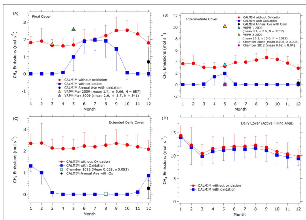
Figure 4: Measured and modeled average monthly CH 4 emissions ( \text{mol s}^{-1} ) for individual cover areas. (A) Final Cover (soil only, negligible emissions from final cover with geomembrane), (B) Intermediate Cover, (C) Extended Daily Cover, (D) Active Filling Area (thin overnight daily cover). DOI: https://doi.org/10.1525/elementa.145.f4
