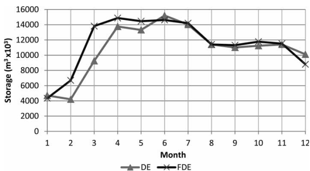
Figure 7 | Wildwood reservoir storage for a 12 month time horizon.
