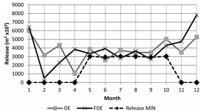
Figure 8 | Wildwood reservoir release for a 12 month time horizon.
