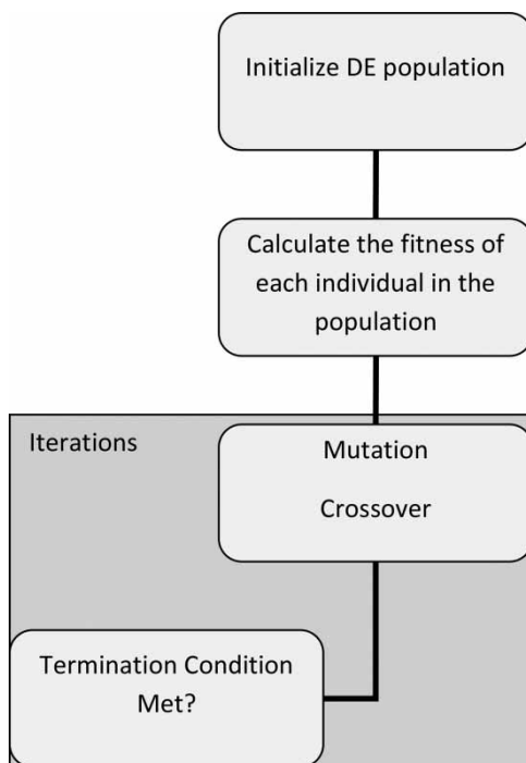
Figure 1 | DE algorithm schematic.
