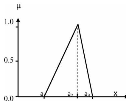
Figure 2 | Triangular fuzzy membership function.
