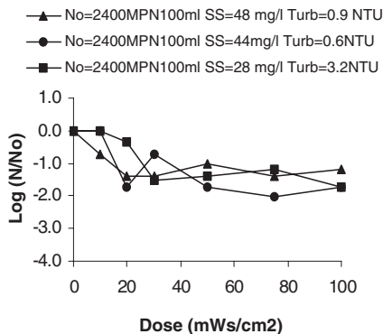
Figure 3 Disinfection of Salmonella with UV irradiation from tertiary effluents filtered to reach different levels of turbidity
