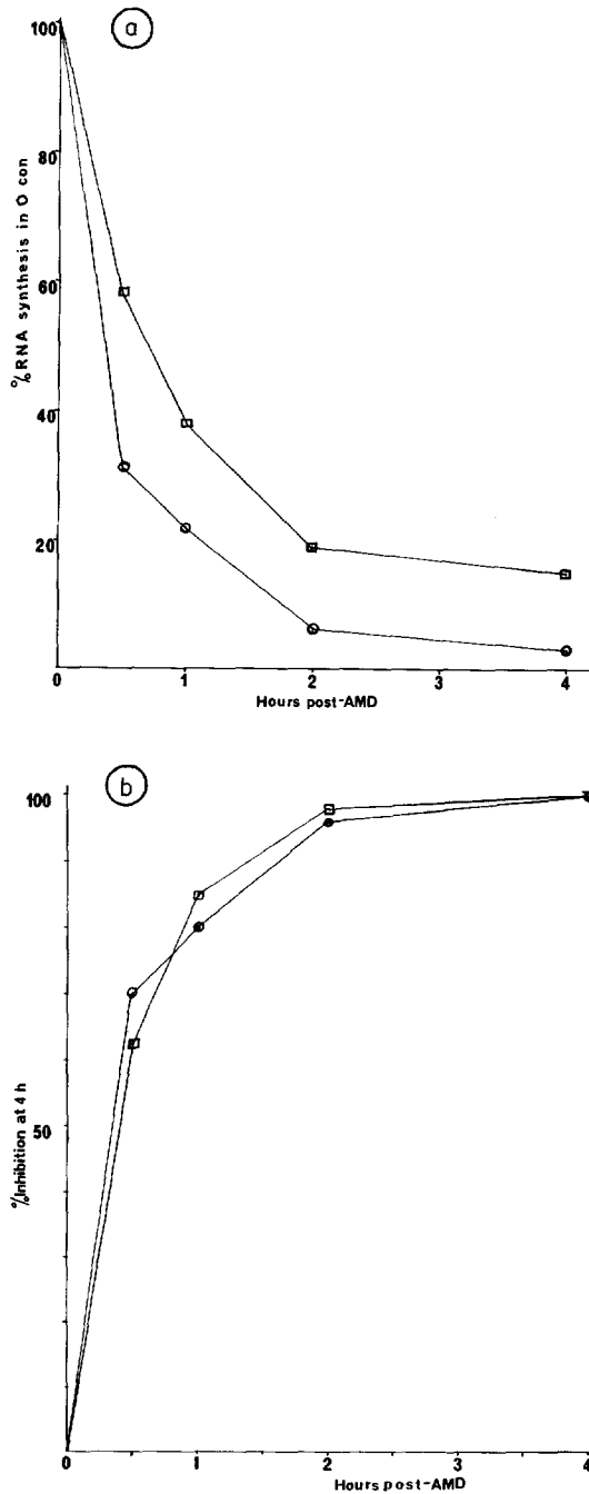
FIGURE 5 Effect of AMD pretreatment on RNA synthesis in normal and transformed cells. AMD (0.25 \mu g/ml) was added to replicate cultures at 0 h, and [ 3 H]uridine was added at times shown. Cultures were incubated for 30 min after addition of [ 3 H]uridine, and then harvested as described in Methods. BHK, —○—; BHK-PV, —□—. (a) The ordinate is a plot of percent RNA synthesis compared with a culture that was labeled for 30 min in the absence of AMD. (b) The ordinate is a plot derived from the same data as 5 a but expressing percent inhibition, taking the inhibition at 4 h as 100%.
