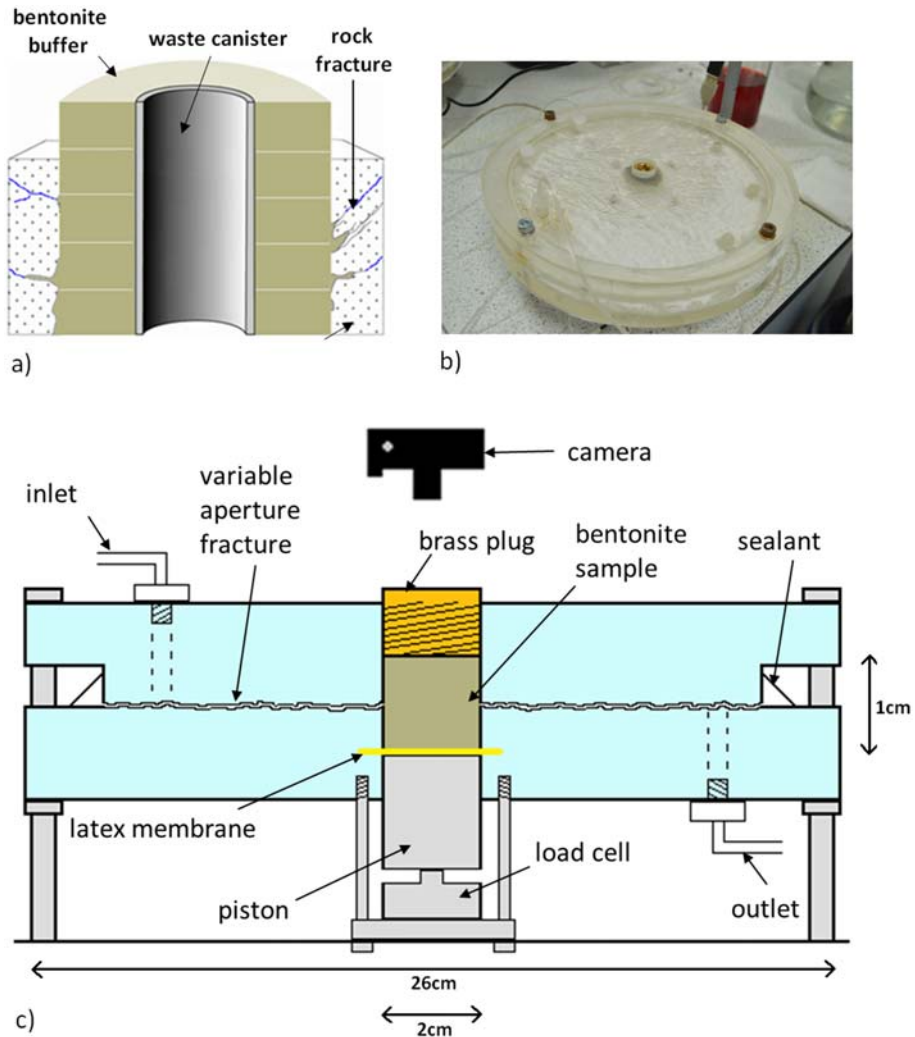
FIG. 1. (a) Cross-section of deposition hole; (b) image of experimental apparatus; (c) schematic cross-section of flow cell.
