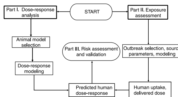
Figure 1 | The QMRA project progressed in three parts. Part 1 involved animal selection and dose response modeling. Part 2 involved the evaluation of human exposures for selected outbreaks with relatively well-documented LD infection rates. Part 3 (the current manuscript) provides a comparison of the QMRA model risk predictions with the outbreak's disease risks.
