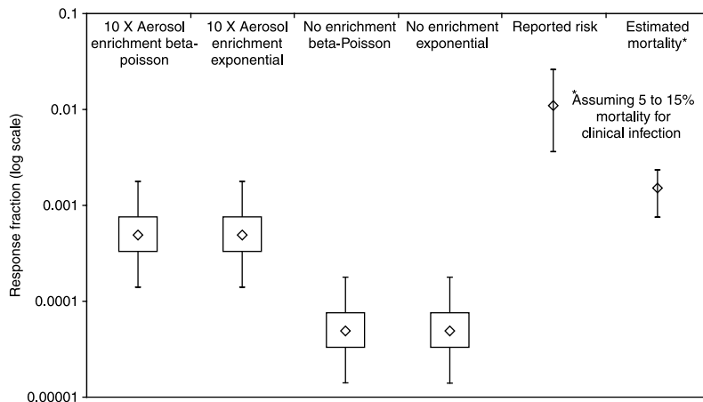
Figure 5 | Comparison of the calculated clinical severity risk with the reported clinical infection risk and estimated mortality risk for the West Frisian outbreak worker group at greater than 15 metres from the whirlpool spa. Bar ends = 2.5 and 97.5th percentiles, box ends = 25 and 75th percentiles, \diamond = median.
