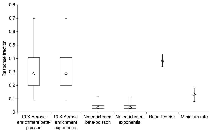
Figure 3 | Comparison of the calculated risks to the reported sub-clinical infection risks (including updated minimum risks) for the West Frisian outbreak worker group at greater than 15 metres from the whirlpool spa. Bar ends = 2.5 and 97.5th percentiles, box ends = 25 and 75th percentiles, ◇ = median.
