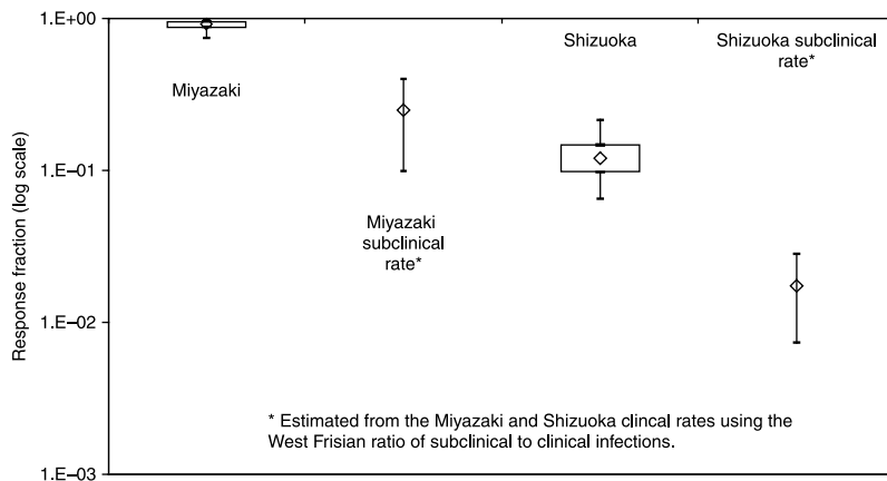
Figure 7 | Comparison of the calculated sub-clinical infection risk with estimated sub-clinical infection risks for the Miyazaki and Shizuoka prefecture outbreaks. Bar ends = 2.5 and 97.5th percentiles, box ends = 25 and 75th percentiles, ◇ = median.
