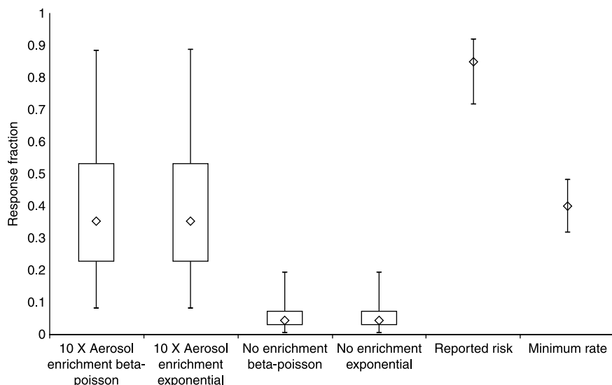
Figure 2 | Comparison of the calculated risks to the reported sub-clinical infection risk and updated minimum infection risks for the West Frisian outbreak worker group at less than 15 metres from the whirlpool spa. Bar ends = 2.5 and 97.5th percentiles, box ends = 25 and 75th percentiles, ◇ = median.
