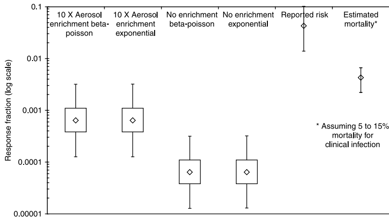
Figure 4 | Comparison of the calculated clinical severity risk with the reported clinical infection risk and estimated mortality risk for the West Frisian outbreak worker group at less than 15 metres from the whirlpool spa. Bar ends = 2.5 and 97.5th percentiles, box ends = 25 and 75th percentiles, \diamond = median.
