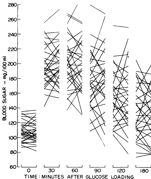
FIG. 1. Reproducibility of 100 gm. oral glucose tolerance tests in thirty mild diabetics. The test was repeated on the same individual within one week. The left end of each line represents the result of the first test and the right end represents that of the second test of the same subject.
