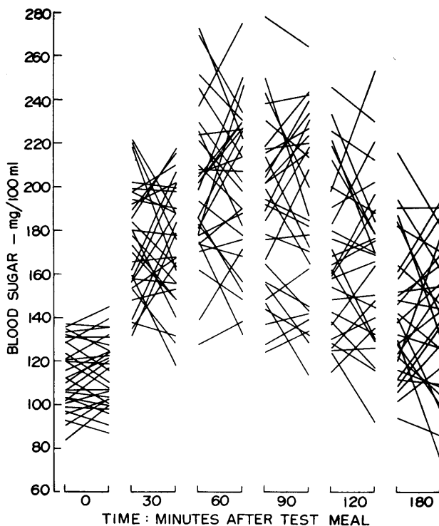
FIG. 2. Reproducibility of Sakaguchi's rice-meal test in thirty mild diabetic patients. The test was repeated twice on the same individual within one week. The left end of each line represents the result of the first test and the right end represents that of the second test of the same subject.
