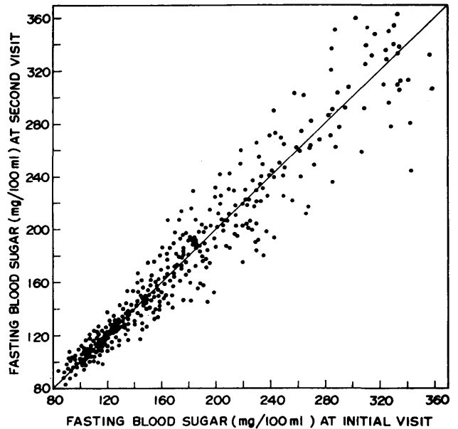
FIG. 3. Variability of fasting blood sugar levels of diabetics determined repeatedly within one-week interval.
