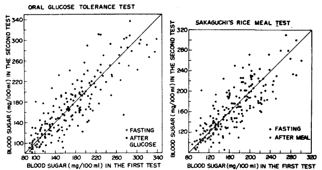
FIG. 4. Comparison of corresponding blood sugar levels in duplicate 100 gm. oral glucose tolerance tests or duplicate Sakaguchi's rice-meal tests.
