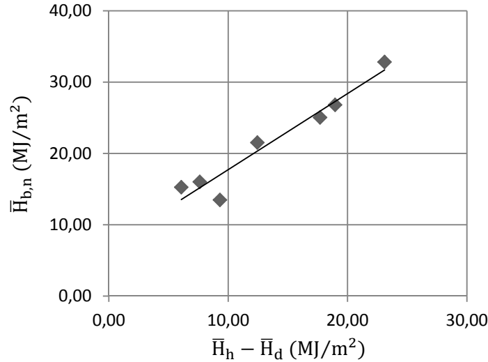
FIGURE 3. Measured \bar{H}_{b,n} ( \text{MJ}/\text{m}^2 ) as function of \bar{H}_h - \bar{H}_d ( \text{MJ}/\text{m}^2 ).
