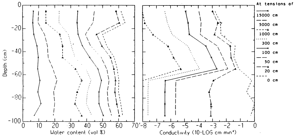
Fig. 3. Soil moisture characteristics (left) and unsaturated conductivity (right) assumed in the simulation.
