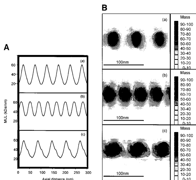
Figure 4. Mean axial mass distributions of microfibrils. Mean axial mass distributions of intact unstained microfibrils were determined from dark-field STEM images using low-dose electron exposure. (A) Axial mass distributions of (a) untreated microfibrils, (b) 5 mM EDTA-treated microfibrils, and (c) 5 mM CaCl 2 -treated microfibrils. (B) Contour plots of axial mass distribution of (a) untreated microfibrils, (b) 5 mM EDTA-treated microfibrils, and (c) 5 mM CaCl 2 -treated microfibrils.
