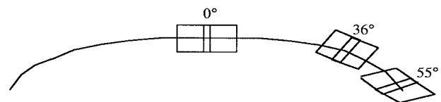
FIG. 10. Footprint rotation with scan is illustrated for three different scan angles. Two adjacent overlapping pixels (scan direction) are shown in each case.
