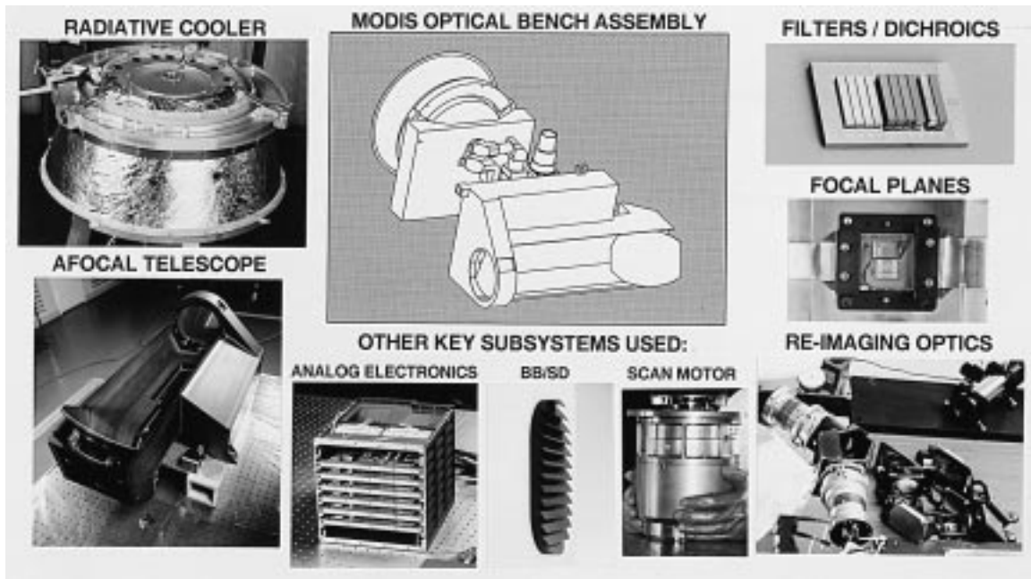
FIG. 5. The Optical Bench Assembly includes the majority of the optical hardware required for the next-generation MODIS. Additional applicable MODIS hardware includes the analog electronics, onboard blackbody, solar diffuser, and scan motor encoder.
