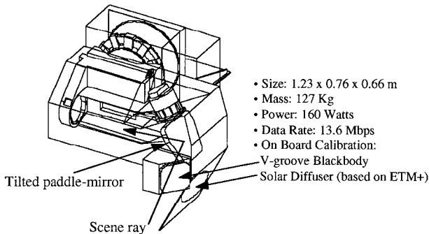
FIG. 8. Minimum size is attained by redesigning the scan subsystem, as shown on the right. A tilted paddle-mirror directs scene energy into the OBA aperture.
