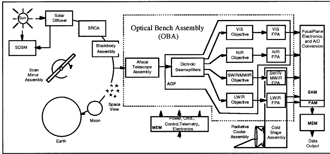
FIG. 4. The Optical Bench Assembly comprises the afocal telescope, the refractive objectives, focal planes, and radiative cooler.
