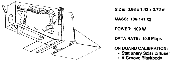
FIG. 7. Baseline scan MODIS Light option preserves baseline paddle-wheel scan, as well as blackbody and solar diffuser (top) and space view.
