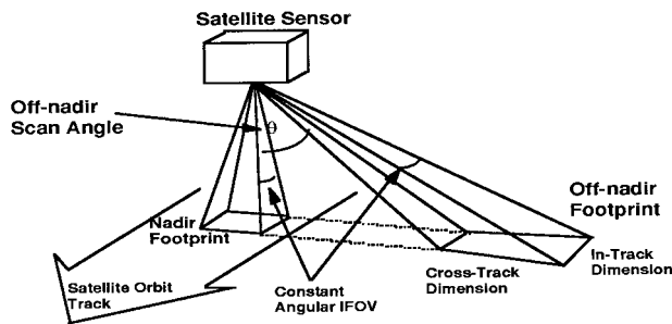
FIG. 3. The NPOESS day/night cloud imagery horizontal spatial resolution (HSR) requirement sets in-track and cross-track HSR at 400 m nadir and 800 m at \theta = 56.5^\circ .
