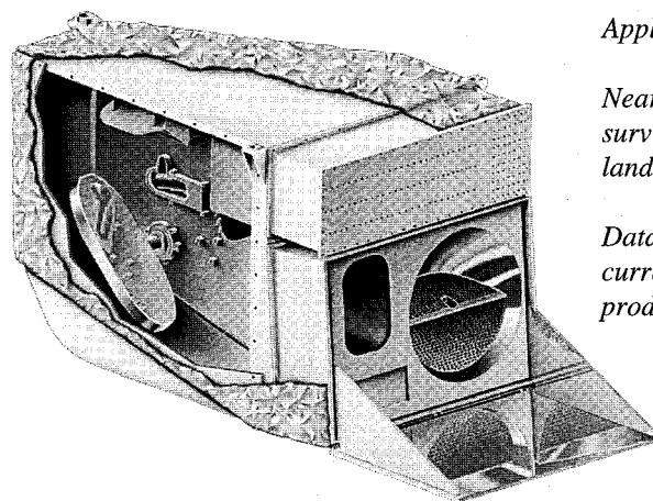
FIG. 1. MODIS artist's conception shows 360° scan mirror required to view multiple onboard calibration systems as well as the earth scene below.
