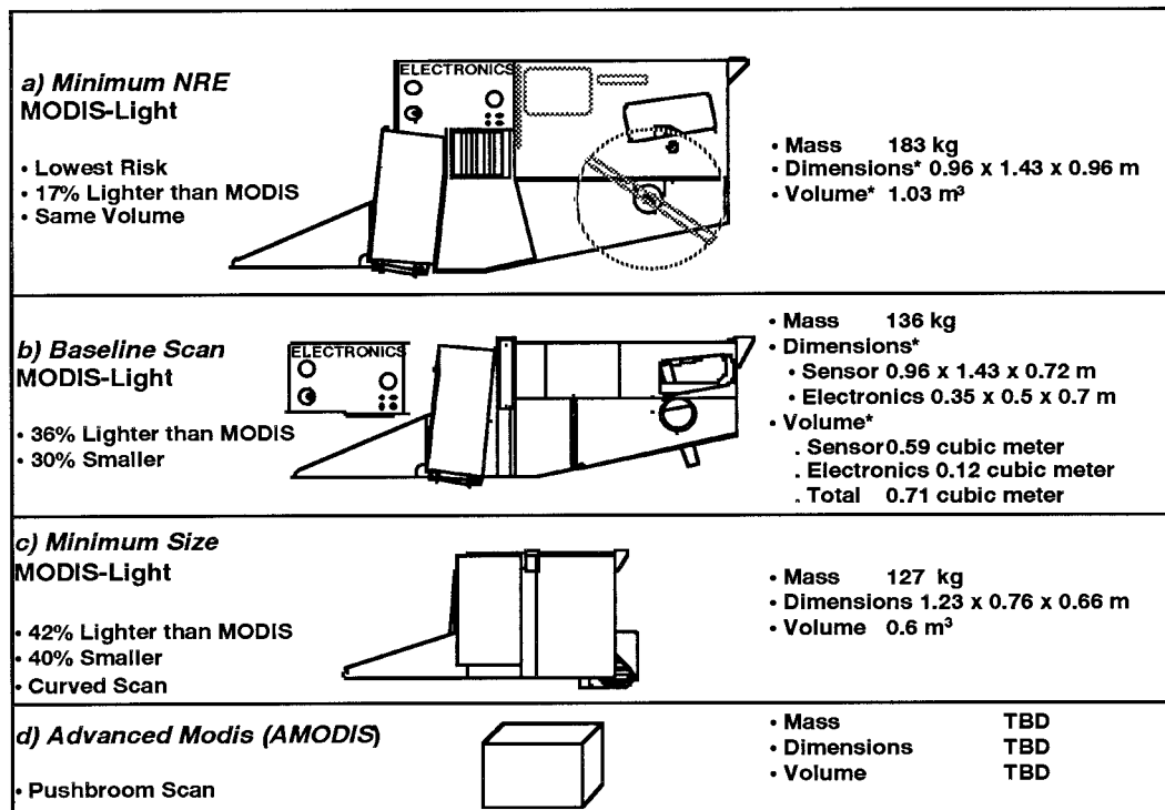
FIG. 6. Four MODIS follow-on options considered. (*Dimensions of a rectangular box that could enclose the instrument in the launch configuration. Actual exterior volume is listed.)
